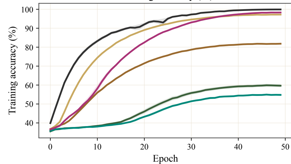
Training accuracy (%)
