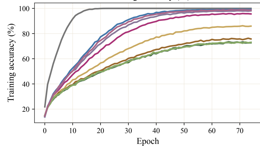
Training accuracy (%)
