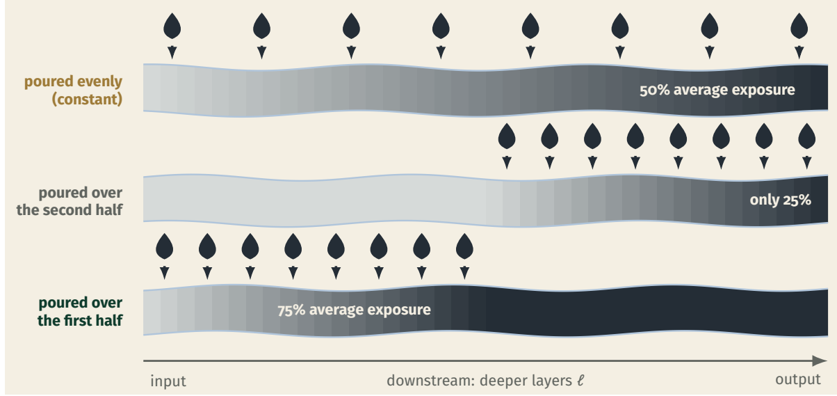
Figure 3. Imagine you have a flowing river and a set amount of ink, with the goal of causing as much corruption as possible at every point: where would you drop it? Framing current dropout practice through this lens makes it clear why front-loading is more effective: the current carries the ink forward.
