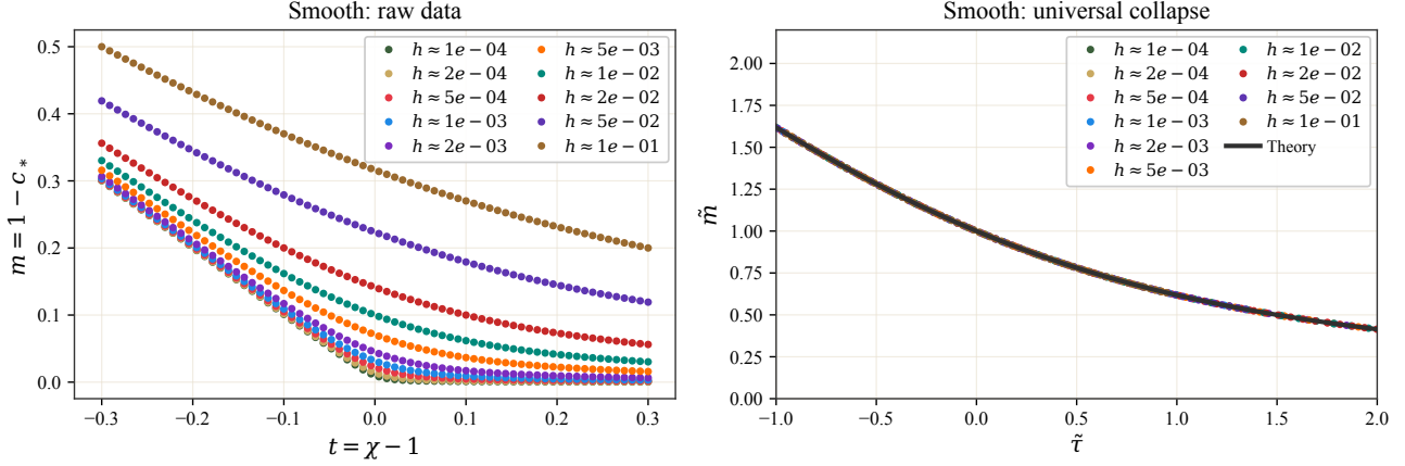
Figure 2. Two-parameter crossover and scaling collapse of the dropout-deformed equation of state for the smooth universality class (tanh). Plots obtained using MFT recursion relations. The figure displays the relationship between different variables collapsing into a universal function as \tilde{\tau} increases. The kinked counterpart is shown in Fig. 4.
