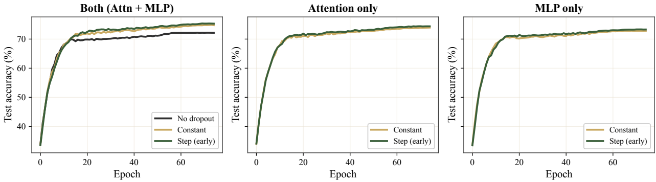
Figure 11. Component ablations applying dropout schedules to the attention block, MLP block, or both. The figure compares no dropout, constant dropout, and step-like dropout.
