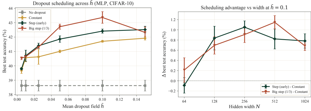
(a) Sweep over mean dropout probability at width N = 256 . (b) Schedule advantage over constant dropout at \bar{p} = 0.1 .
