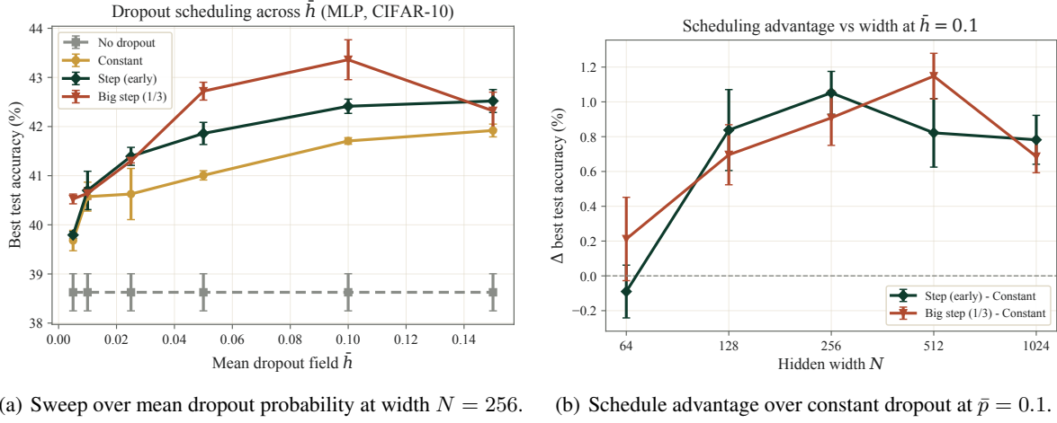
Figure 9. Robustness sweeps for depth-6 near-critical ReLU MLPs on CIFAR-10. Early schedules improve over constant dropout throughout the large-width regime, while N = 64 illustrates the expected finite-width boundary.
