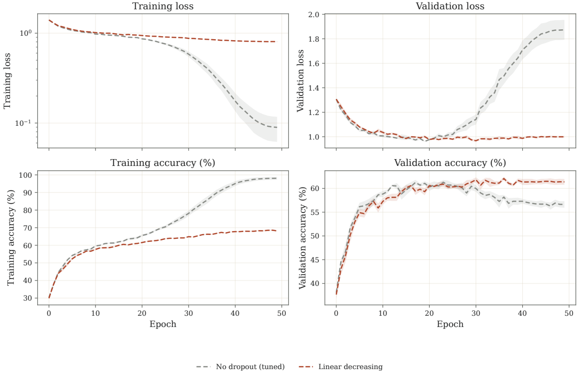
Figure 19. Jannis / Transformer / Linear follow-up. Original-cohort learning curves; bands show SEM across the recorded seeds for each profile. Sample counts and tuned probabilities are given below.
