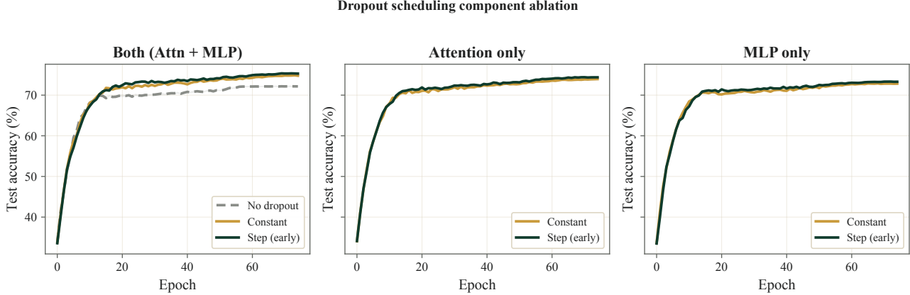
Figure 13. Original five-seed component ablations applying dropout schedules to the attention block, MLP block, or both. The figure compares no dropout, constant dropout, and step-like dropout; it excludes the later both-block seed extension.
