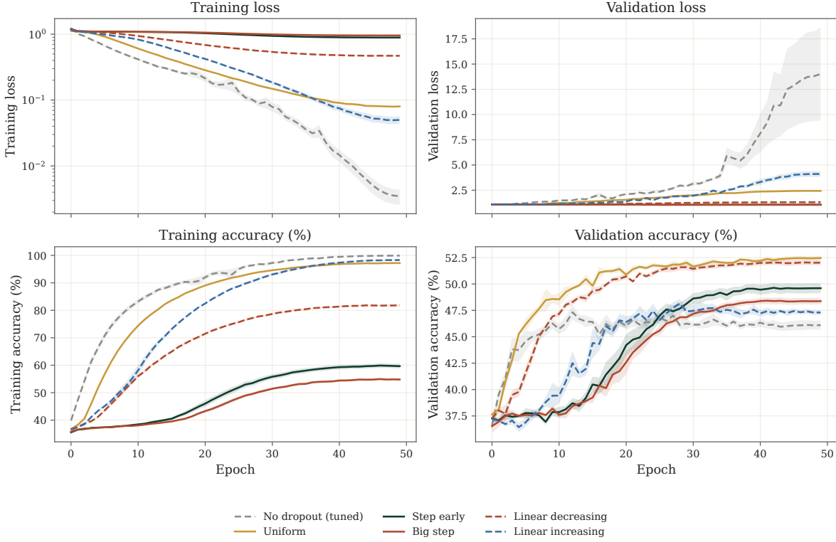
Figure 23. FI-2010 / MLP / Zero weight decay. Original-cohort learning curves; bands show SEM across the recorded seeds for each profile. Sample counts and tuned probabilities are given below.
