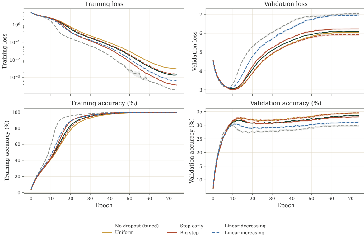
Figure 17. Tiny ImageNet / Transformer / 80,000 train. Original-cohort learning curves; bands show SEM across the recorded seeds for each profile. Sample counts and tuned probabilities are given below.
