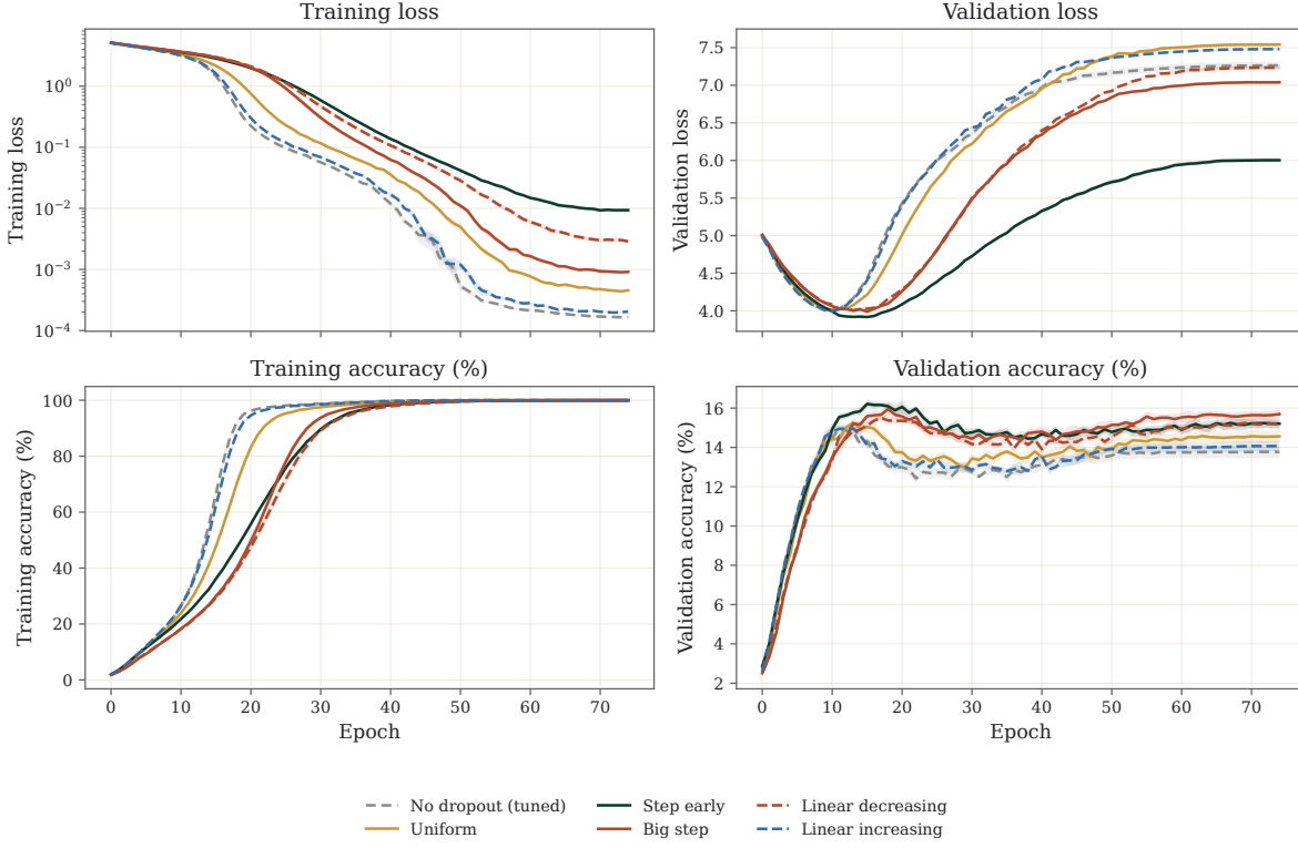
Figure 22. Tiny ImageNet / Transformer / Zero weight decay. Original-cohort learning curves; bands show SEM across the recorded seeds for each profile. Sample counts and tuned probabilities are given below.
