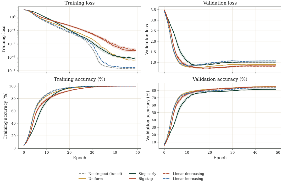
Figure 15. Speech Commands / Transformer / Zero weight decay. Original-cohort learning curves; bands show SEM across the recorded seeds for each profile. Sample counts and tuned probabilities are given below.
