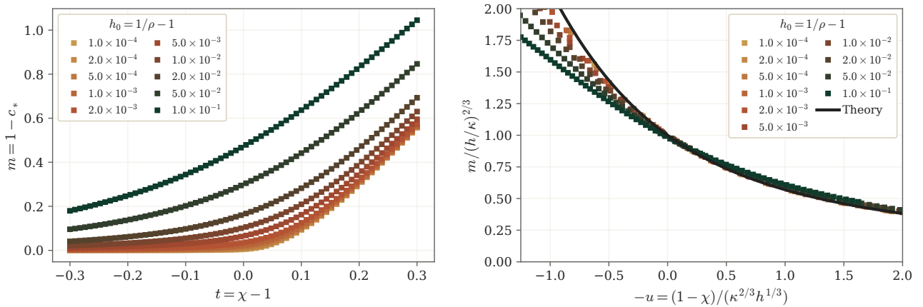
Figure 6. Kinked counterpart to Fig. 2, using the formal ReLU channel above. Each curve fixes h_0 = 1/\rho - 1 , the field at \chi = 1 . Points solve the full map and are rescaled with the actual field h = \chi h_0 and the critical coefficient \kappa = 2\sqrt{2}/(3\pi) . The right panel shows the window 0 \leq m/(h/\kappa)^{2/3} \leq 2 , with horizontal coordinate -u relative to Eq. (38). The black curve is the leading equation of state; departures at finite field include the full map’s \chi -dependent kink coefficient.
