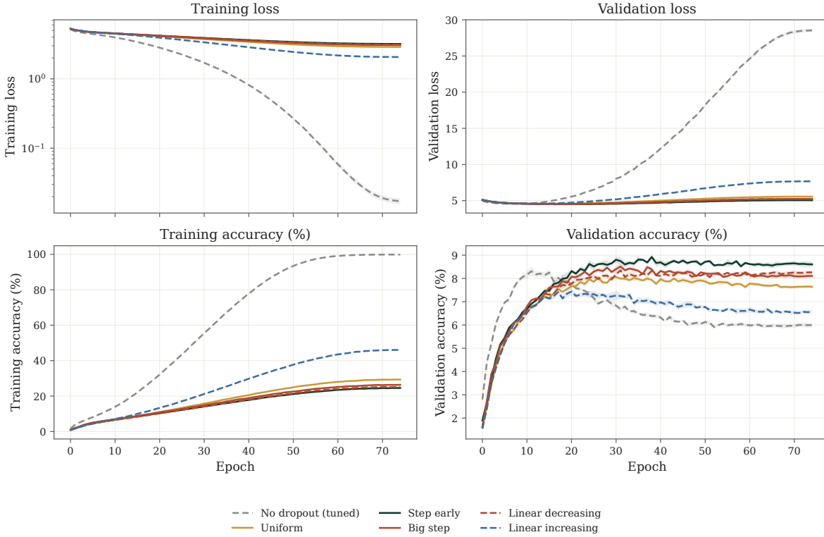
Figure 16. Tiny ImageNet / MLP / 80,000 train. Original-cohort learning curves; bands show SEM across the recorded seeds for each profile. Sample counts and tuned probabilities are given below.
