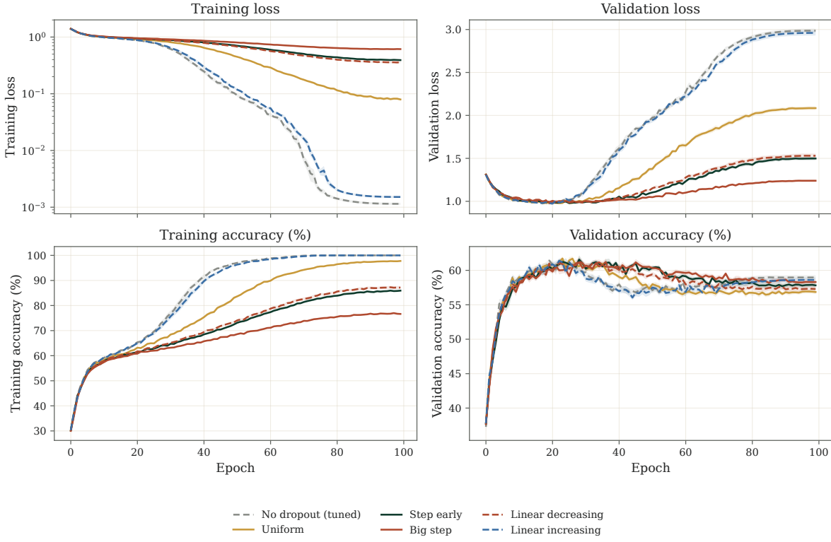
Figure 20. Jannis / Transformer / 100 epochs. Original-cohort learning curves; bands show SEM across the recorded seeds for each profile. Sample counts and tuned probabilities are given below.
