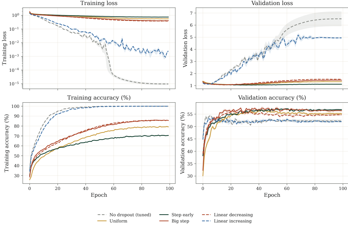
Figure 24. Jannis / MLP / Zero weight decay. Original-cohort learning curves; bands show SEM across the recorded seeds for each profile. Sample counts and tuned probabilities are given below.
