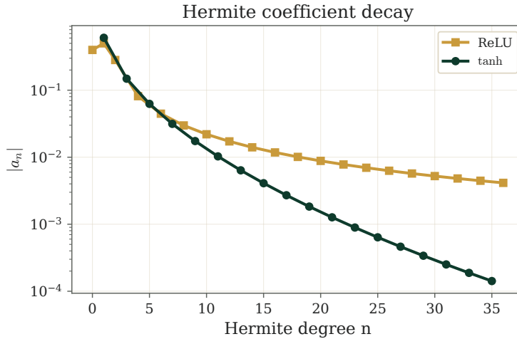
Figure 5. Hermite coefficient magnitudes for the unscaled activations \text{ReLU}(z) and \tanh(z) . The ReLU coefficients use their exact expression; tanh uses 220-point Gauss–Hermite quadrature. The coefficient tail exposes the difference in regularity at c = 1 .
