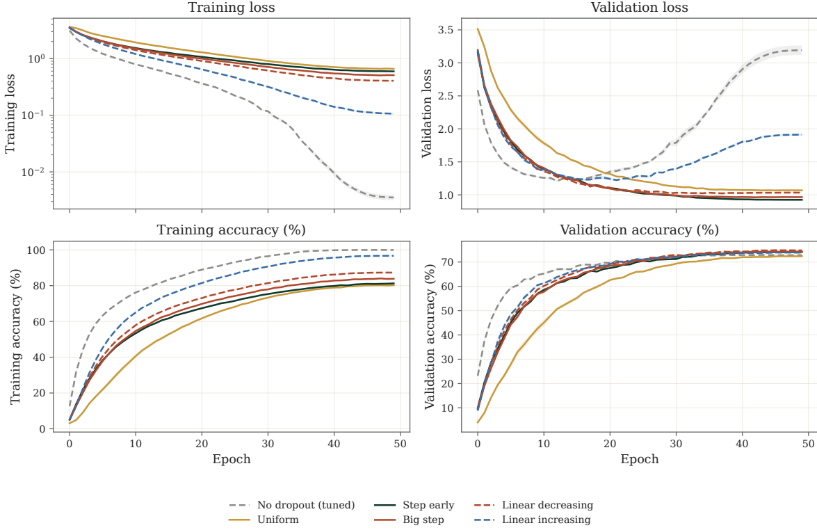
Figure 14. Speech Commands / MLP / Zero weight decay. Original-cohort learning curves; bands show SEM across the recorded seeds for each profile. Sample counts and tuned probabilities are given below.
