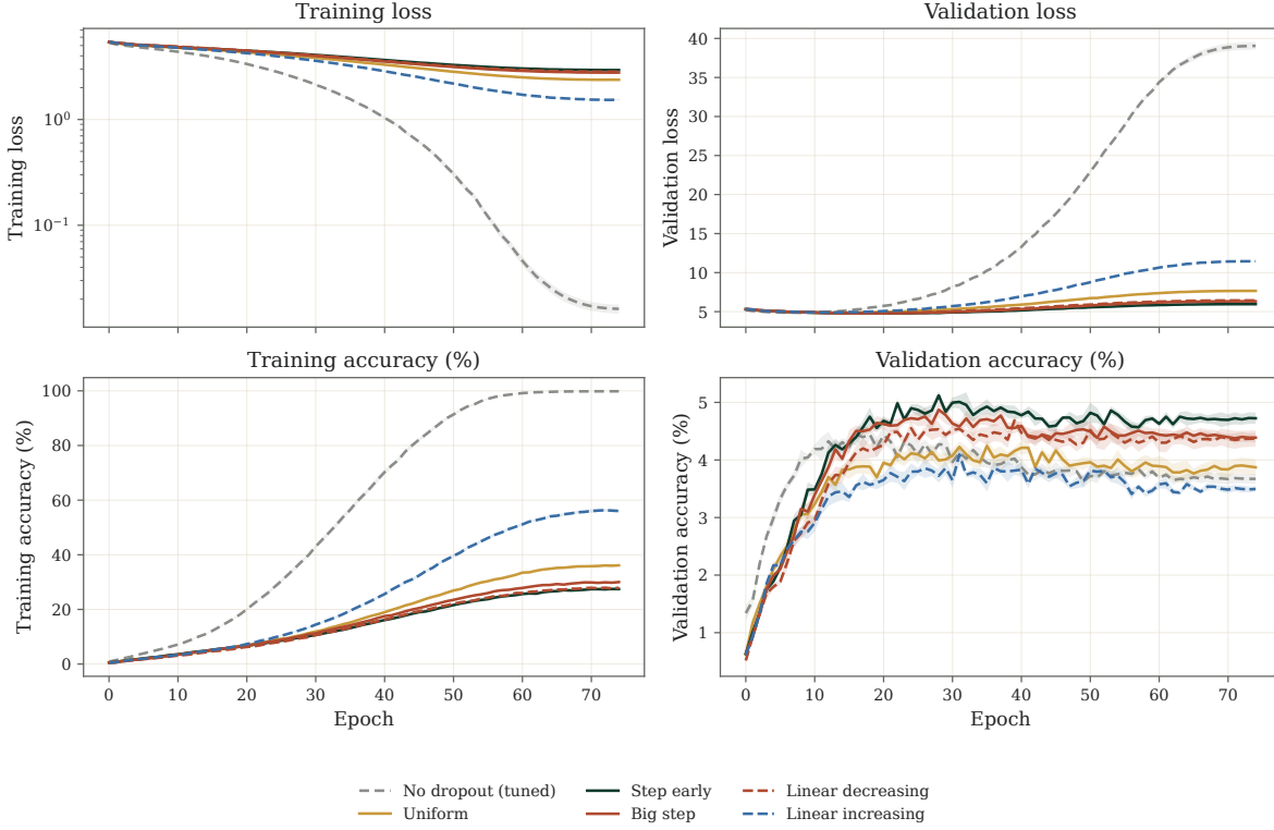
Figure 21. Tiny ImageNet / MLP / Zero weight decay. Original-cohort learning curves; bands show SEM across the recorded seeds for each profile. Sample counts and tuned probabilities are given below.
