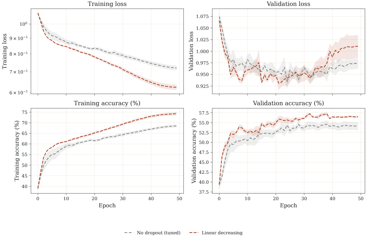
Figure 18. FI-2010 / Transformer / Linear follow-up. Original-cohort learning curves; bands show SEM across the recorded seeds for each profile. Sample counts and tuned probabilities are given below.
