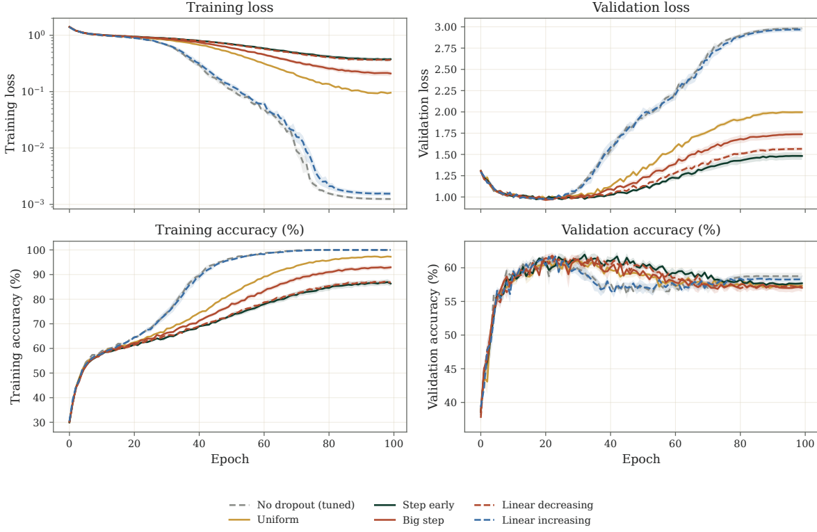
Figure 25. Jannis / Transformer / Zero weight decay. Original-cohort learning curves; bands show SEM across the recorded seeds for each profile. Sample counts and tuned probabilities are given below.
