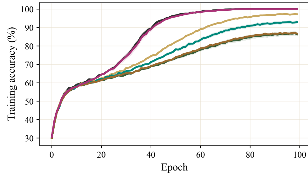
Training accuracy (%)
