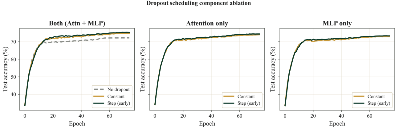
Figure 13. Original five-seed component ablations applying dropout schedules to the attention block, MLP block, or both. The figure compares no dropout, constant dropout, and step-like dropout; it excludes the later both-block seed extension.
