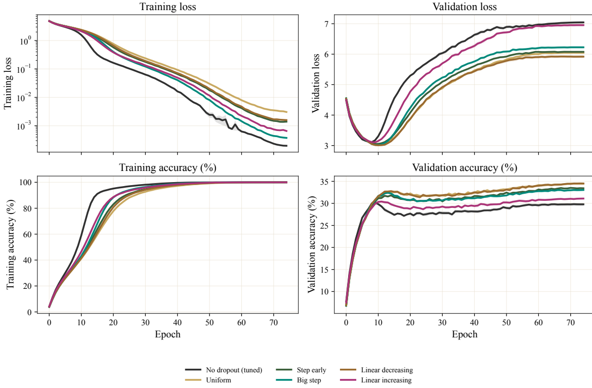
Figure 17. Tiny ImageNet / Transformer / 80,000 train. Original-cohort learning curves; bands show SEM across the recorded seeds for each profile. Sample counts and tuned probabilities are given below.
