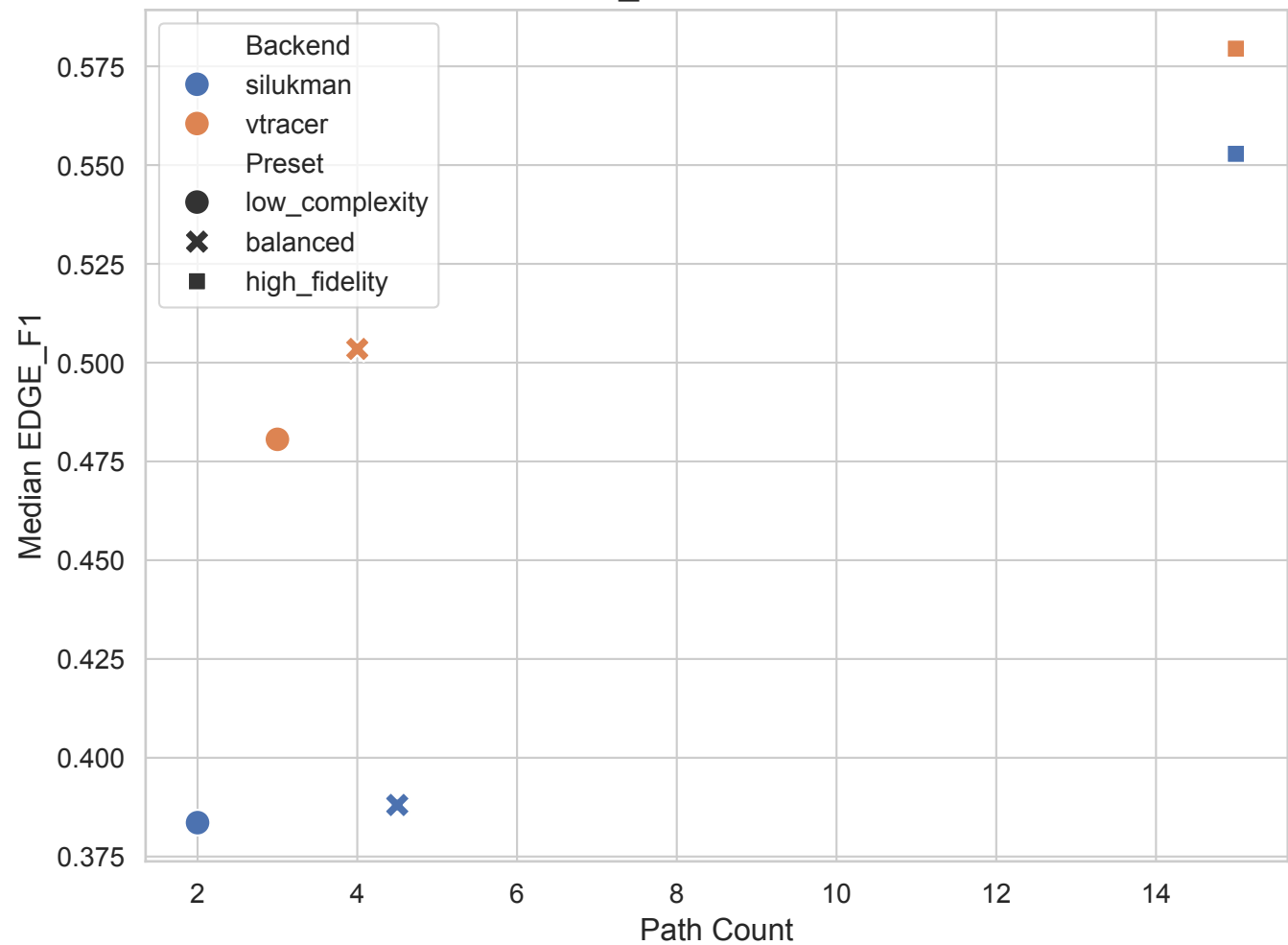
EDGE_F1 vs Path Count
