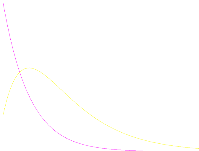
Figure 8.3: Nuclear chain reaction: A decays into B decays into C
