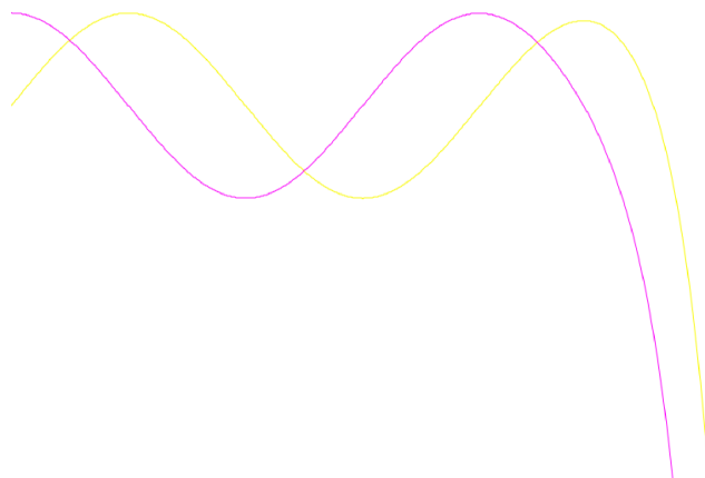
Figure 8.2: Numerical errors in sine/cosine computation
