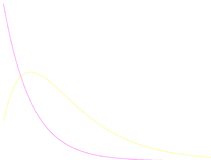
Figure 8.3: Nuclear chain reaction: A decays into B decays into C
