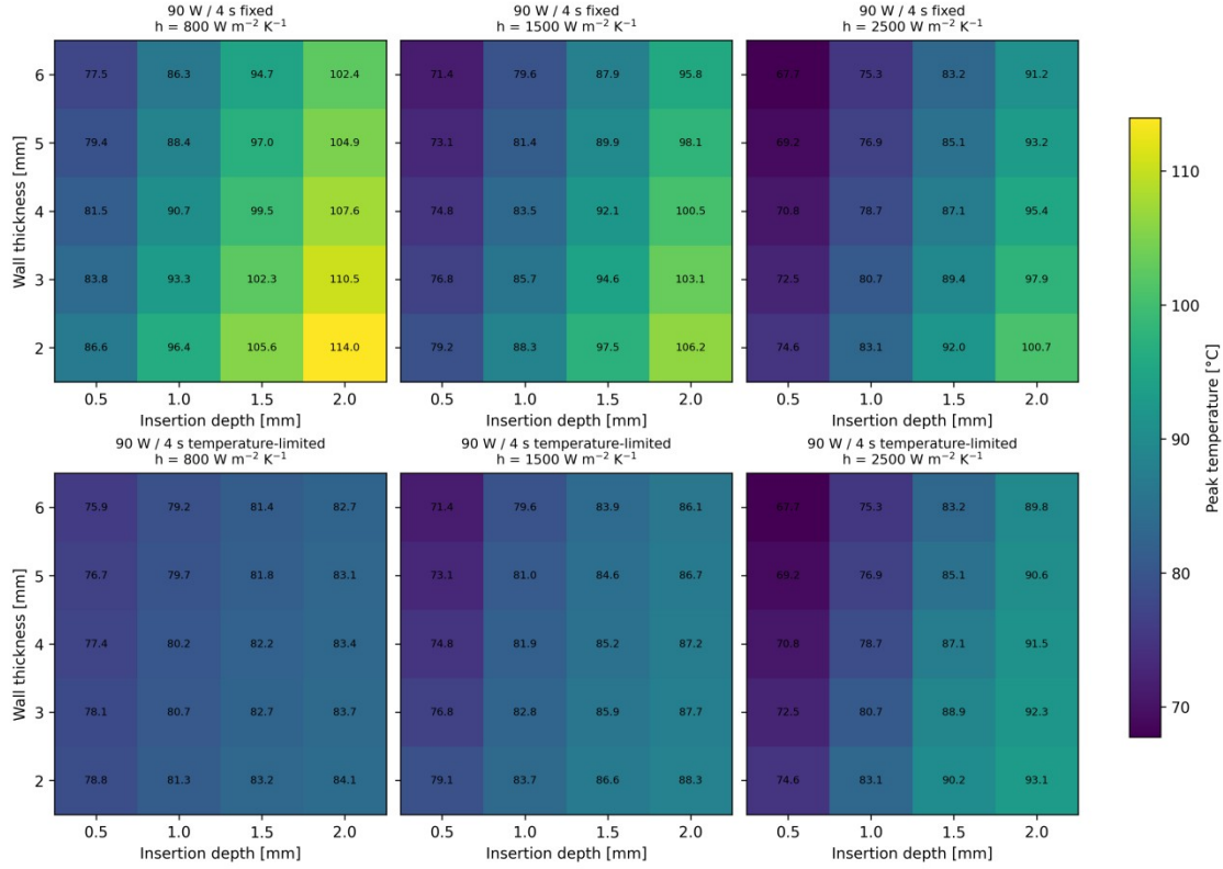
Figure 6. Peak-temperature maps for fixed-power and generic temperature-limited 90 W / 4 s across the phase-preparation grid. Columns correspond to cooling coefficients of 800, 1500, and 2500 \text{W m}^{-2} \text{K}^{-1} ; rows compare the fixed-power and temperature-limited comparators.
