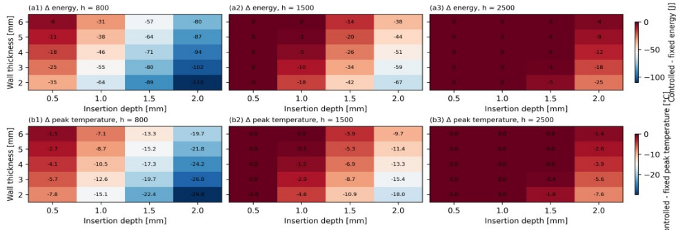
Figure 7. Controlled-minus-fixed difference maps for 90 W / 4 s across the phase-preparation grid. The upper row shows reductions in delivered energy, and the lower row shows reductions in peak temperature, for the generic temperature-limited comparator relative to the fixed-power comparator.
