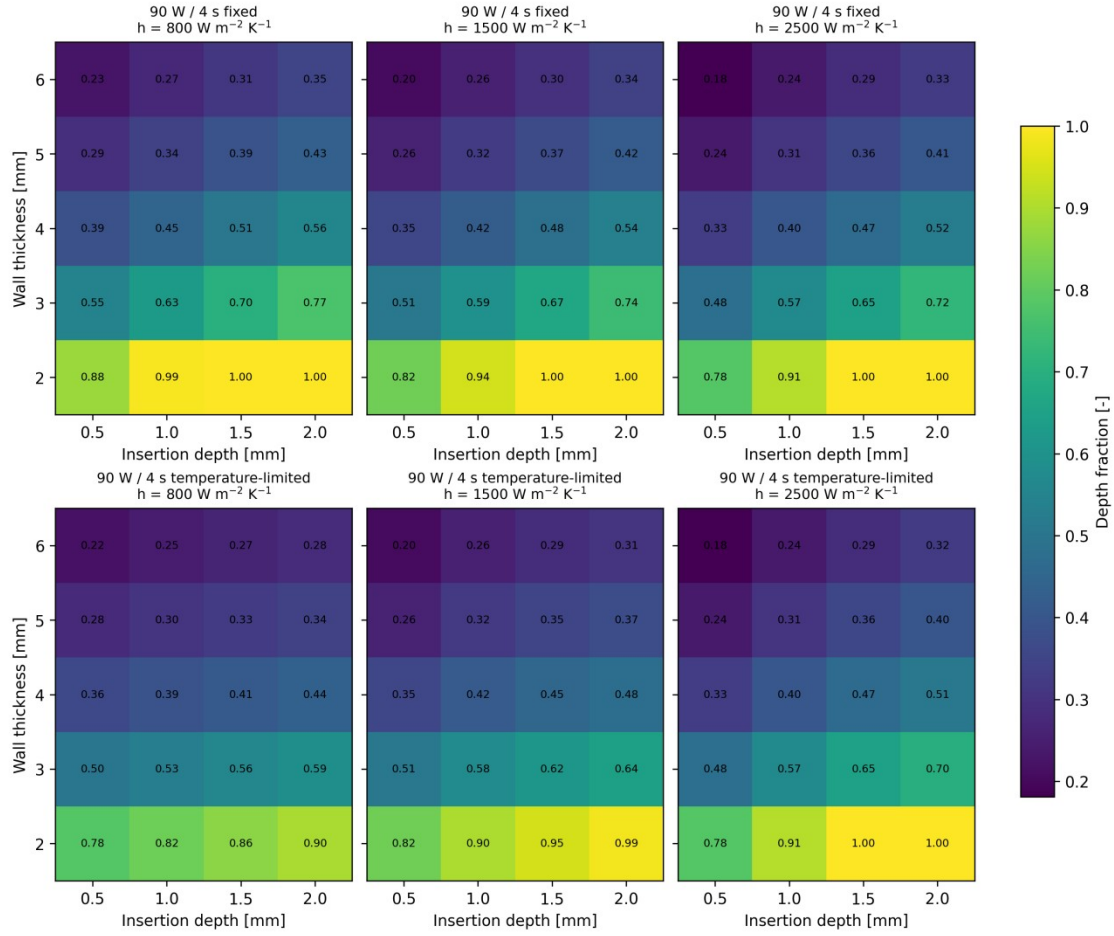
Figure 5. Depth-fraction maps for fixed-power and generic temperature-limited 90 W / 4 s across the phase-preparation grid. Columns correspond to cooling coefficients of 800, 1500, and 2500 W m -2 K -1 ; rows compare the fixed-power and temperature-limited comparators. Values are reported over wall thickness and insertion depth combinations.
