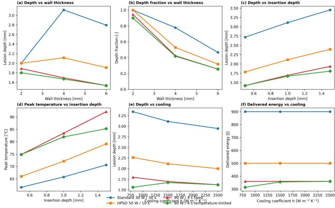
Figure 3. Deterministic four-way comparison across representative wall-thickness, insertion-depth, and cooling slices. Panels summarize lesion depth and depth fraction versus wall thickness, lesion depth and peak temperature versus insertion depth, and lesion depth and delivered energy versus cooling for standard RF, HPSD, fixed-power 90 W / 4 s, and generic temperature-limited 90 W / 4 s.
