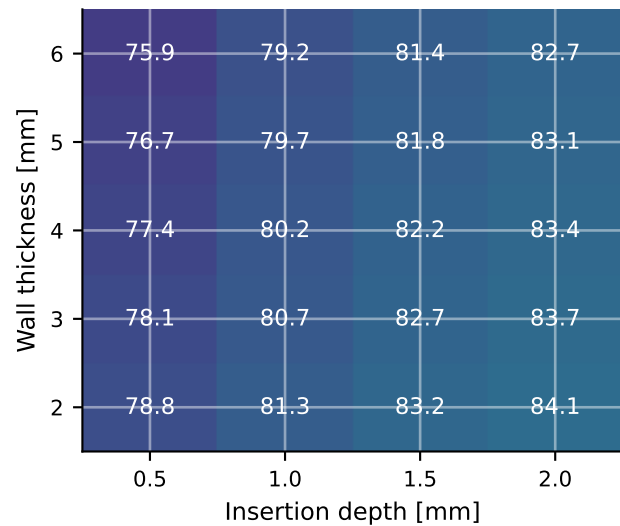
90 W / 4 s temperature-limited
