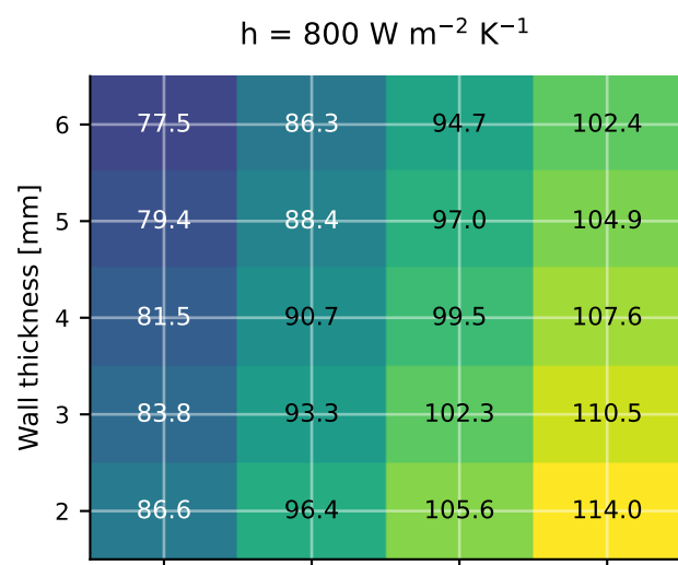
90 W / 4 s fixed
