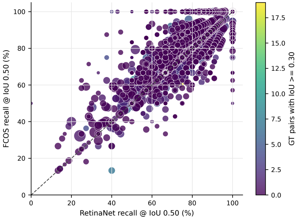
Crowded / overlapped scene recall
