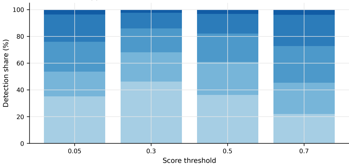
Approximate FPN-level distribution of FCOS detections
