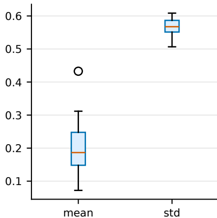
bbox ctrness
