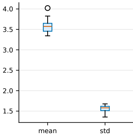
bbox regression
