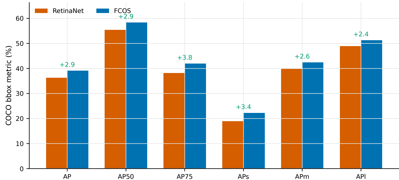
FCOS vs. RetinaNet on COCO val2017
