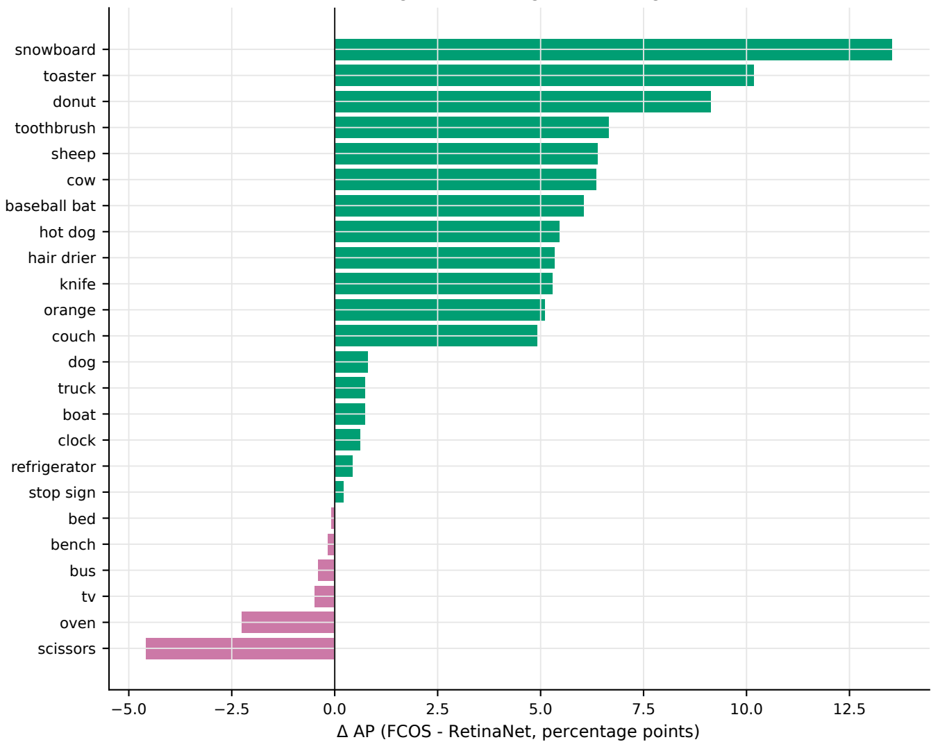
Categories with largest AP changes
