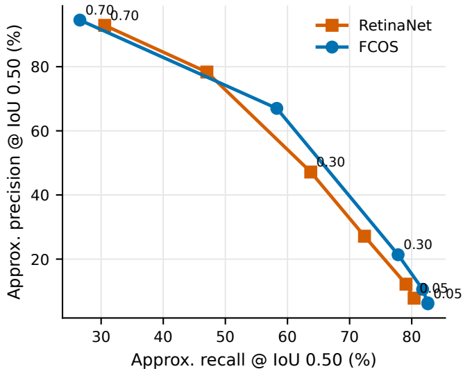
Score-threshold trade-off
