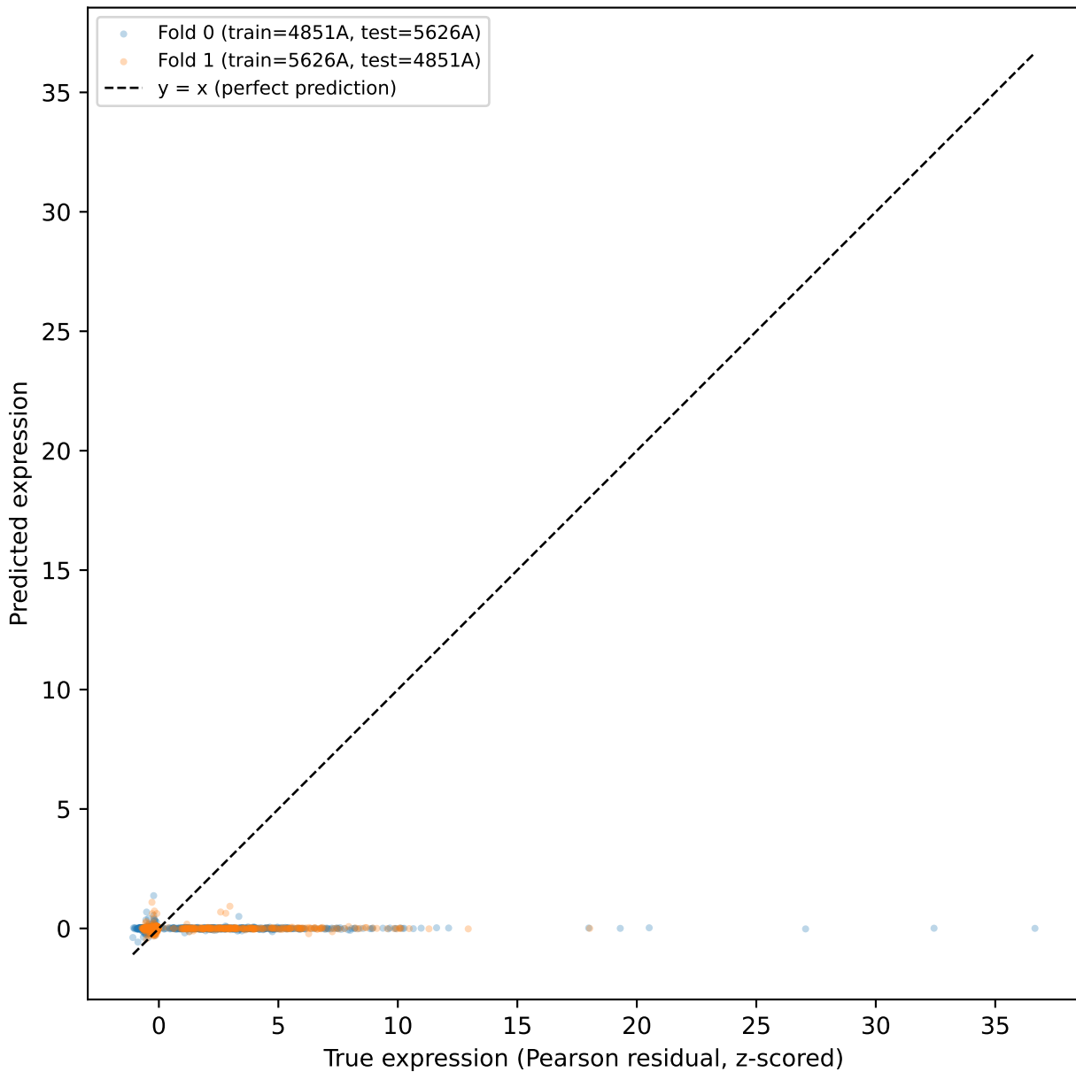
padded: predicted vs true expression (all genes, both folds) overall R = 0.012, n = 10000 sampled points
