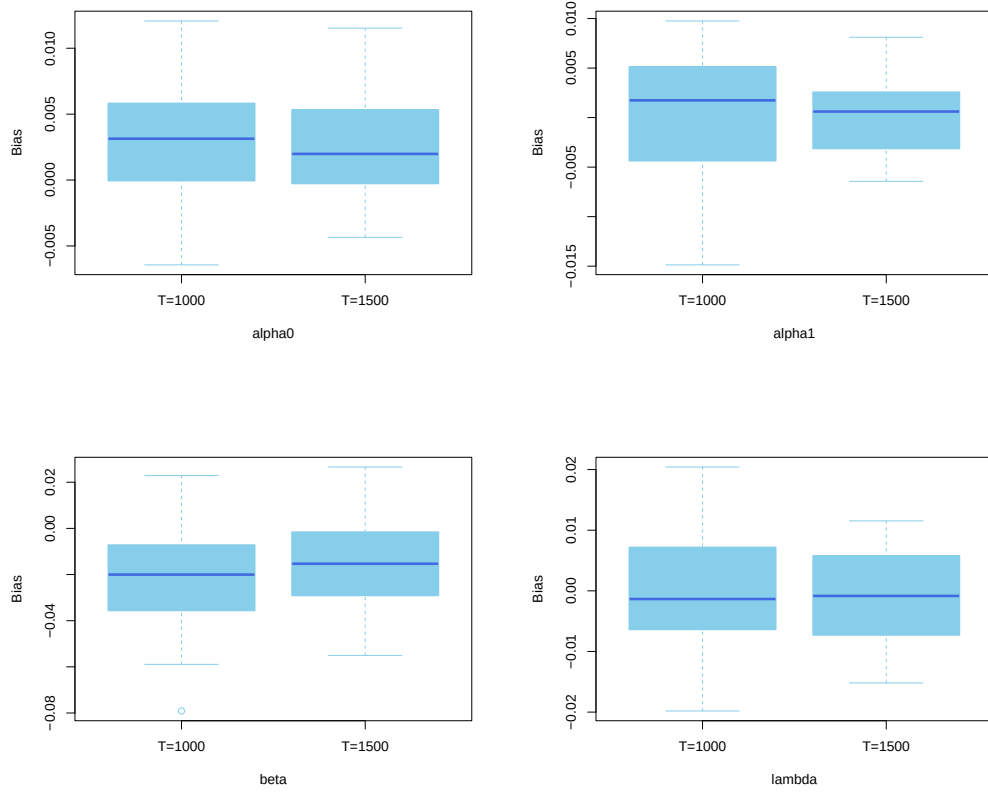
Figure 2. Boxplots of bias for \hat{\theta}_{iT,\tau} at \tau = 0.1 , for normal innovations, where \alpha_0 , \alpha_1 , \beta and \lambda represent corresponding elements of \hat{\theta}_{\tau T}
