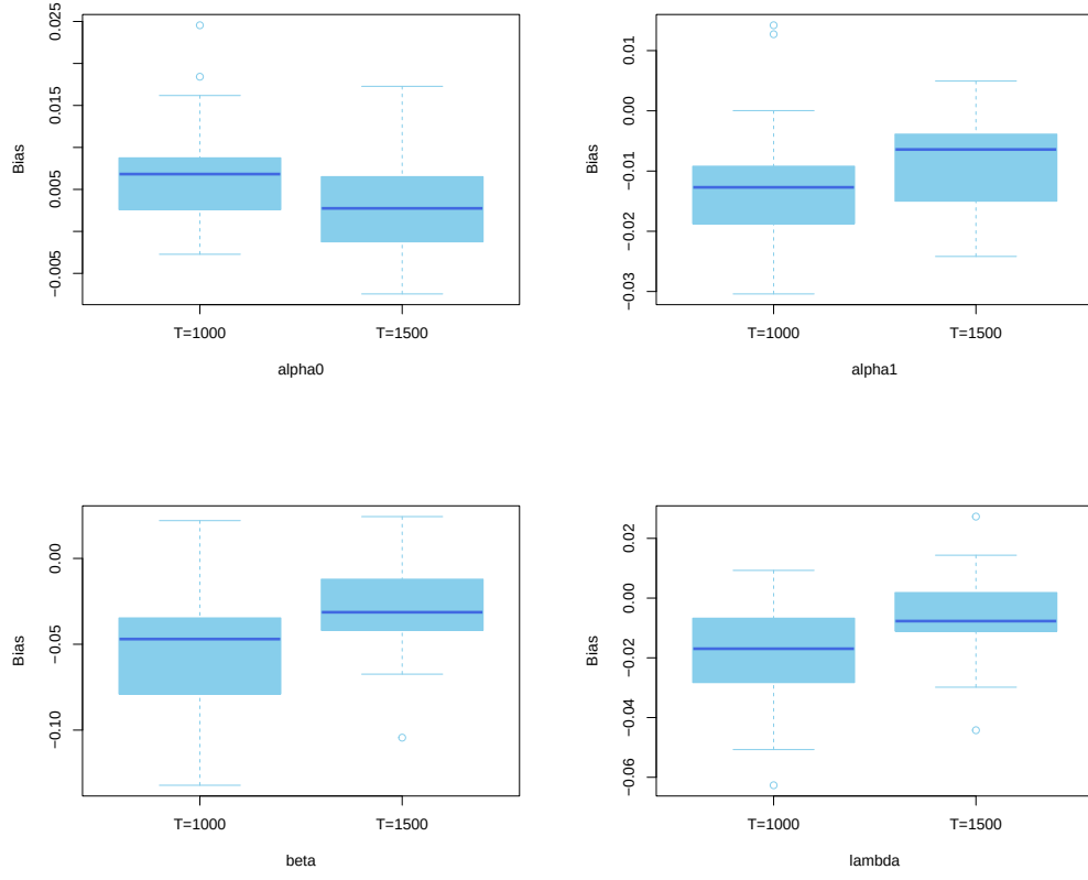
Figure 3. Boxplots of bias for \hat{\theta}_{iT,\tau} at \tau = 0.05 , for Student t_5 -distributed innovations, where \alpha_0 , \alpha_1 , \beta and \lambda represent corresponding elements of \hat{\theta}_{\tau T}
