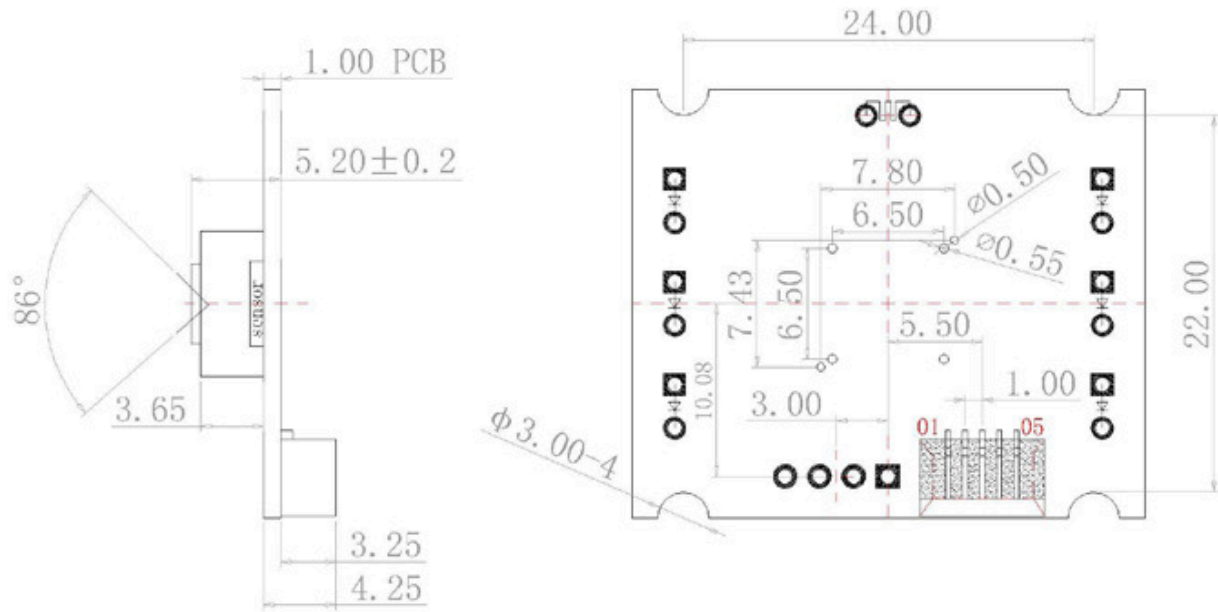
TOP VIEW
