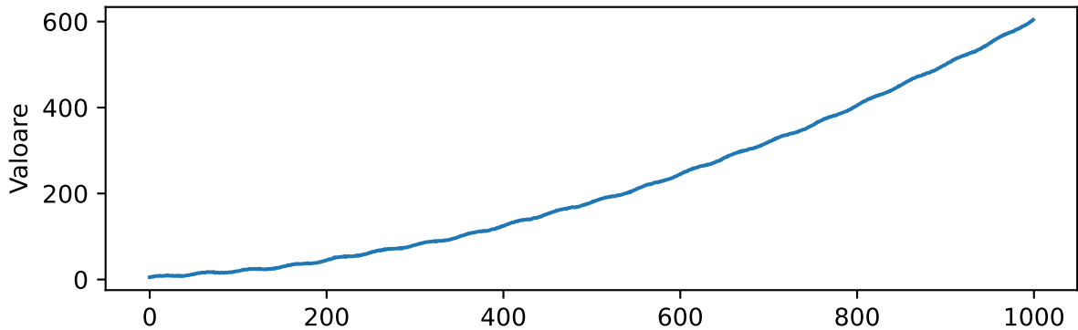
Time series originala
