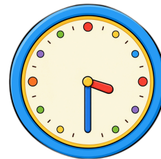
half past
