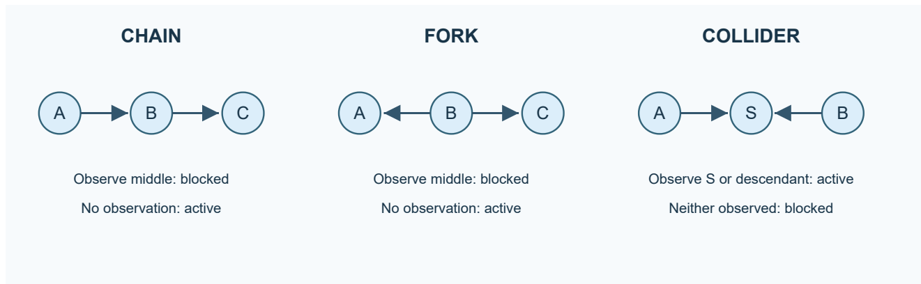
Figure 1. Original teaching diagram of standard d-separation motifs; definitions follow Murphy, §4.2.4. The statements refer to the displayed path and must be checked across all paths in a larger graph.
