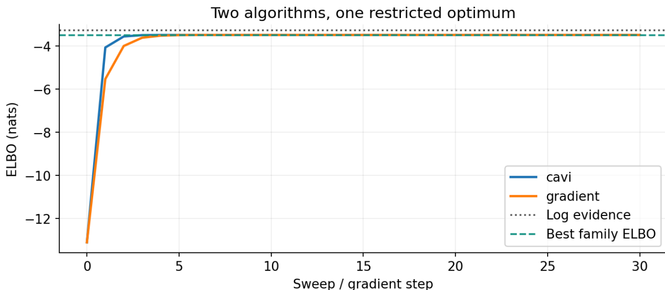
Figure 4. Both algorithms approach the same family optimum. At \rho = .8 , log evidence is -3.277181 , best ELBO is -3.489521 , and irreducible reverse KL is .212340 nats. Negative ELBO values are expected here.
