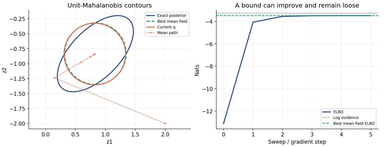
Figure 2. These are unit-Mahalanobis contours, not 68% joint credible regions. Rotation represents covariance. An axis-aligned approximation cannot reproduce it even after its center converges.
