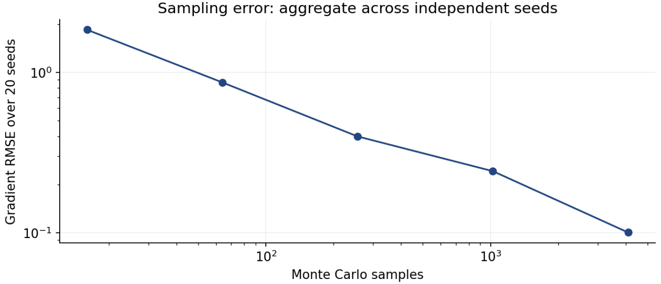
Figure 5. Root mean squared gradient error is aggregated over 20 independent seeds for each sample count. More samples reduce typical error, but a particular realization need not improve monotonically. This plot measures gradient-estimation error, not posterior approximation error.
