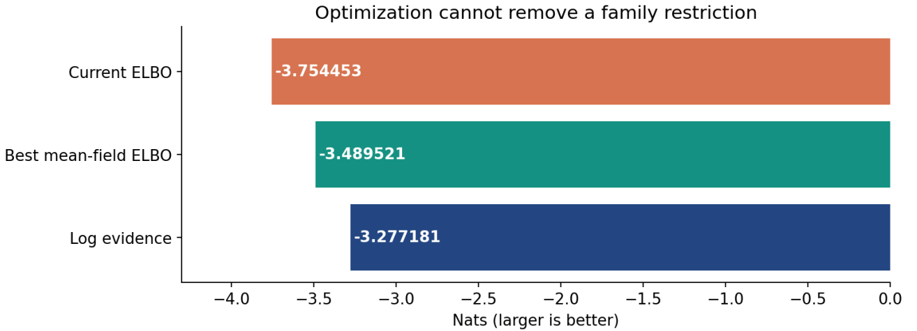
Figure 1. Two distinct gaps are visible. Increasing iterations can reduce the optimization gap; it cannot enlarge a fixed family. All values come from the independently implemented synthetic model below.
