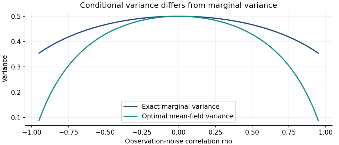
Figure 3. At \rho = 0 , the posterior factorizes and the gap vanishes. Away from zero, missing dependence matters. The horizontal axis is noise correlation.
