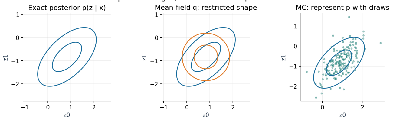
F01 | Same target; two different representations
