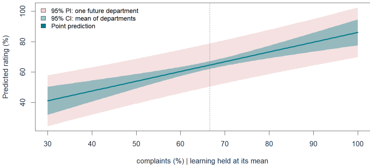
Same center, two different uncertainty targets
