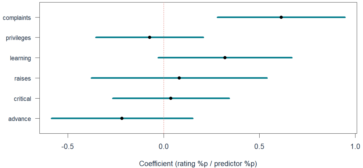
Six-predictor model: point estimates and 95% CIs
