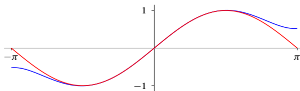
Graphs on [-\pi, \pi] of the sine function (red) and the Taylor polynomial (blue) from 6.70.
