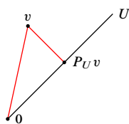
P_U v is the closest point in U to v .
