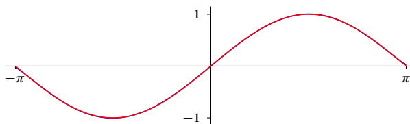
Graphs on [-\pi, \pi] of the sine function (red) and its best fifth degree polynomial approximation u (blue) from 6.69.
