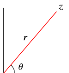
Representation of a complex number with polar coordinates.
