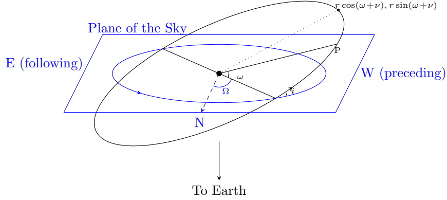
Figure 1: In this North becomes the local X axis and West becomes the Y axis of the sky plane.
