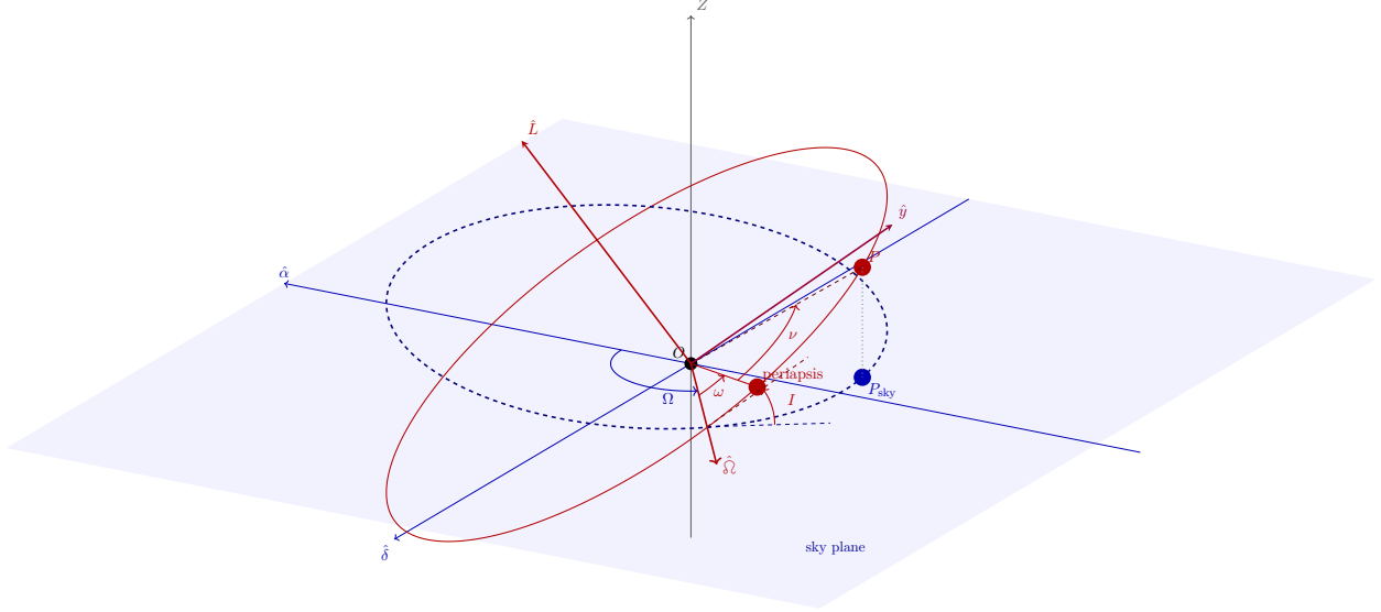
Figure 2: Orientation of an orbit relative to sky plane. \Omega (longitude of ascending node) is measured from the reference direction \alpha to the ascending node along the sky plane; \omega (argument of periapsis) is measured from the ascending node to perigee within the orbital plane; \iota (inclination) is the dihedral angle between the two planes, read off at the node; \nu (true anomaly) is measured from perigee to the heavenly body's current position. This is exactly (\Omega, \iota, \omega) of Eqs. (5)–(6) describe.
