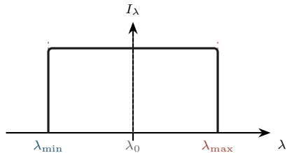
(b) Observed line profile
