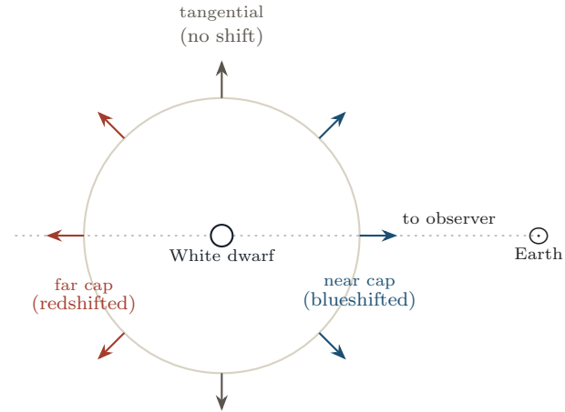
(a) Expanding shell, as seen from Earth
