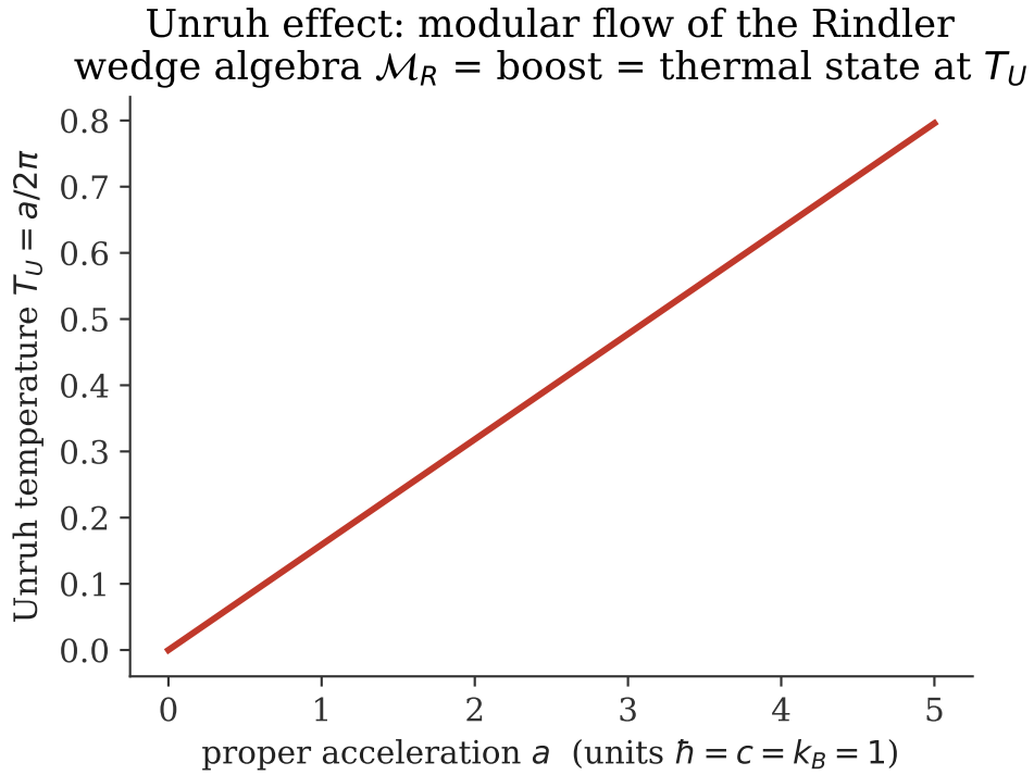
Figure 7: The Bisognano–Wichmann theorem and the Unruh effect: the modular flow \sigma_t^\Omega(A) = \Delta_\Omega^{it} A \Delta_\Omega^{-it} acting on the right Rindler wedge \mathcal{M}_R is geometrically equivalent to a Lorentz boost with parameter \eta = 2\pi t . Accelerated observers perceive the Minkowski vacuum as a thermal KMS state with local Unruh temperature T(x) = \hbar c / (2\pi k_B x) .
