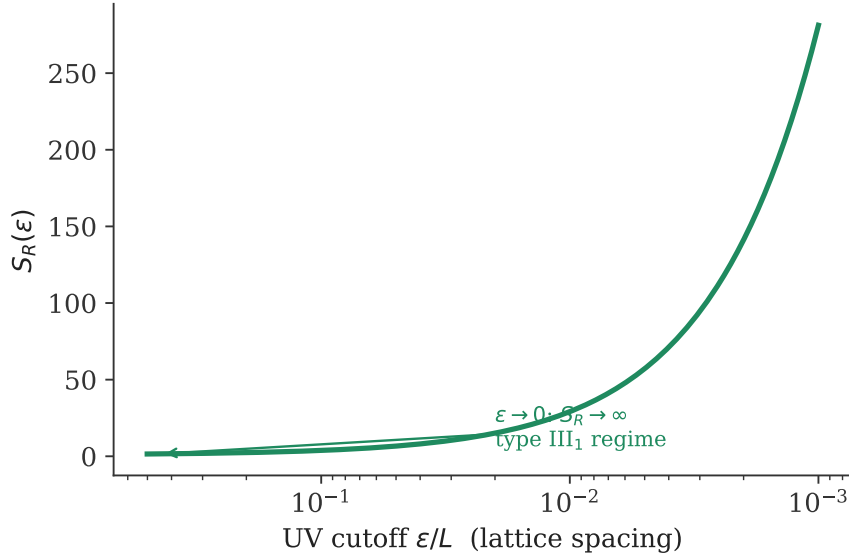
Figure 3: The UV area-law divergence of entanglement entropy in quantum field theory: dividing space across a boundary \partial R couples short-distance modes across the cut with UV cutoff \epsilon . The leading entanglement entropy diverges as S_R \sim \text{Area}(\partial R)/\epsilon^{d-2} , reflecting the infinite entanglement of the underlying Type \text{III}_1 local algebra.
