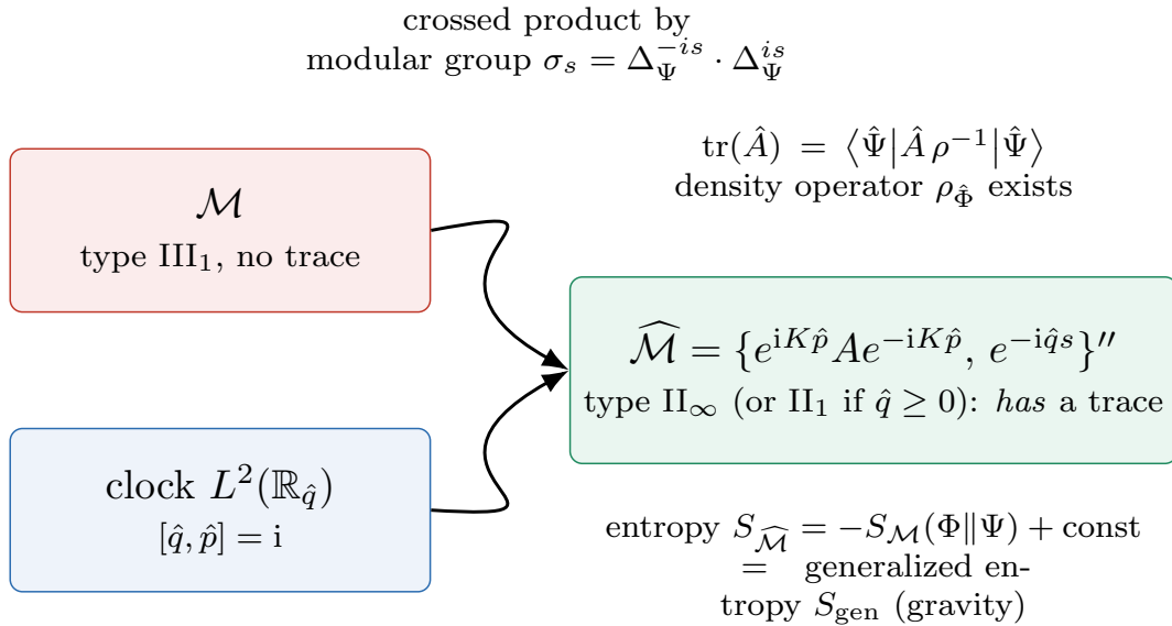
Figure 8: The crossed product construction: crossing a Type \text{III}_1 algebra \mathcal{M} (which has no trace) with its modular automorphism group \sigma_s = \Delta_\Psi^{-is} \cdot \Delta_\Psi^{is} via an auxiliary quantum observer clock L^2(\mathbb{R}) generates a Type \text{II}_\infty factor \widehat{\mathcal{M}} = \mathcal{M} \rtimes_\sigma \mathbb{R} . The resulting algebra supports a well-defined trace \tau , density matrices, and finite generalized entropy S_{\text{gen}} .
