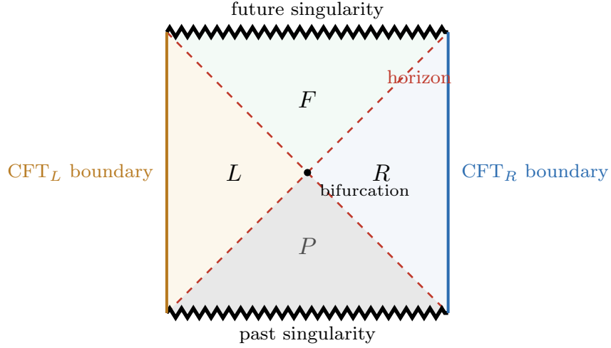
Figure 9: Penrose diagram of the two-sided eternal AdS black hole dual to the Thermofield Double state |\Psi_\beta\rangle . The right ( R ) and left ( L ) exterior wedges are causally disconnected and bounded by the event horizons (dashed red lines), connected in the interior by an Einstein–Rosen bridge (wormhole) between the past ( P ) and future ( F ) curvature singularities (zigzag lines).
