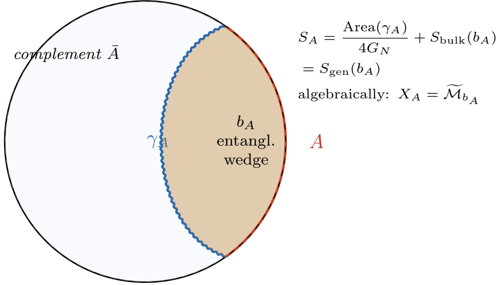
Figure 10: Subregion–subalgebra duality in AdS/CFT: for a boundary subregion A , the Ryu–Takayanagi minimal surface \gamma_A bounds the bulk entanglement wedge b_A . The boundary algebra X_A is isomorphic to the bulk von Neumann algebra \widetilde{\mathcal{M}}_{b_A} . The holographic entanglement entropy is given by S(A) = \frac{\text{Area}(\gamma_A)}{4G_N} + S_{\text{bulk}}(b_A) = S_{\text{gen}}(b_A) .
