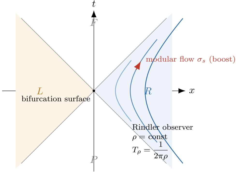
Figure 6: The spacetime geometry of the Rindler wedge: Minkowski spacetime split into the Right wedge R ( x > |t| ), Left wedge L ( x < -|t| ), Future F , and Past P . The boost hyperbolae x^2 - t^2 = \rho^2 represent trajectories of uniformly accelerated observers with proper acceleration a = 1/\rho , whose proper time \tau = \rho\eta is governed by the boost parameter \eta .
