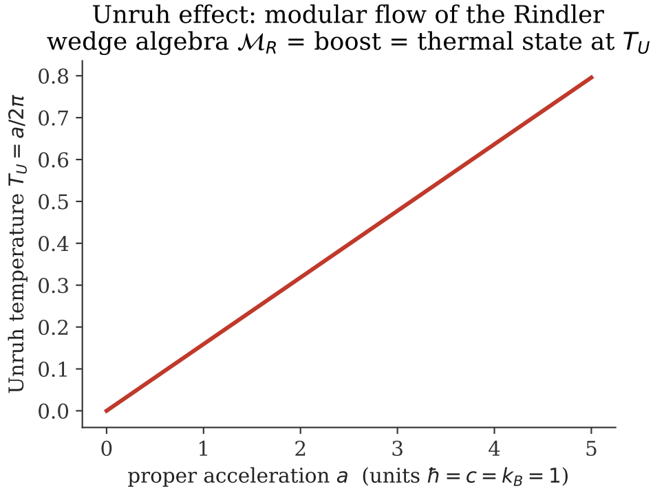
Figure 8: The Bisognano–Wichmann theorem and the Unruh effect: the modular flow \sigma_t^\Omega(A) = \Delta_\Omega^{it} A \Delta_\Omega^{-it} acting on the right Rindler wedge \mathcal{M}_R is geometrically equivalent to a Lorentz boost with parameter \eta = 2\pi t . Accelerated observers perceive the Minkowski vacuum as a thermal KMS state with local Unruh temperature T(x) = \hbar c / (2\pi k_B x) .
