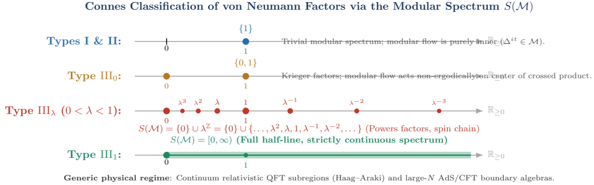
Figure 6: Connes’ modular spectrum classification of von Neumann factors. The invariant S(\mathcal{M}) \equiv \bigcap_\Psi \text{Spec}(\Delta_\Psi) \subset \mathbb{R}_{\geq 0} characterizes the factor type: Types I and II have trivial spectrum \{1\} ; Type \text{III}_0 has \{0, 1\} ; Type \text{III}_\lambda ( 0 < \lambda < 1 ) forms a discrete geometric ladder \{0\} \cup \lambda^{\mathbb{Z}} (Powers factors); and Type \text{III}_1 fills the entire non-negative continuum [0, \infty) (relativistic QFT subregions and large- N holography).
