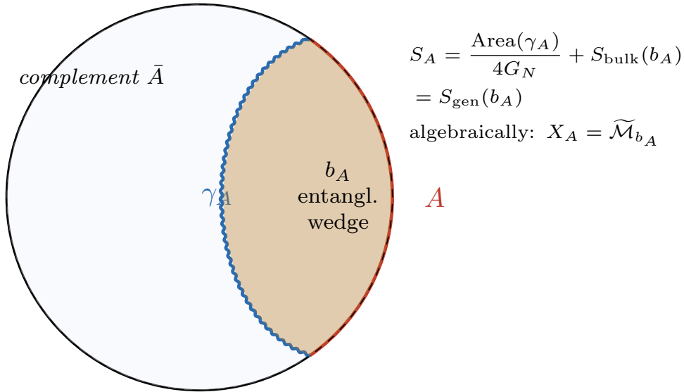
Figure 11: Subregion–subalgebra duality in AdS/CFT: for a boundary subregion A , the Ryu–Takayanagi minimal surface \gamma_A bounds the bulk entanglement wedge b_A . The boundary algebra X_A is isomorphic to the bulk von Neumann algebra \widetilde{\mathcal{M}}_{b_A} . The holographic entanglement entropy is given by S(A) = \frac{\text{Area}(\gamma_A)}{4G_N} + S_{\text{bulk}}(b_A) = S_{\text{gen}}(b_A) .
