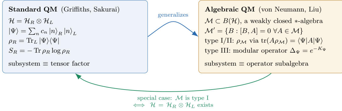
Figure 1: The foundational paradigm shift: Standard Hilbert space quantum mechanics (left, where subsystems are defined by tensor factors \mathcal{H} = \mathcal{H}_R \otimes \mathcal{H}_L ) generalizes to Algebraic Quantum Mechanics (right, where subsystems are defined by operator subalgebras \mathcal{M} \subset B(\mathcal{H}) ). Type I algebras represent the familiar special case where a tensor product factorization exists.
