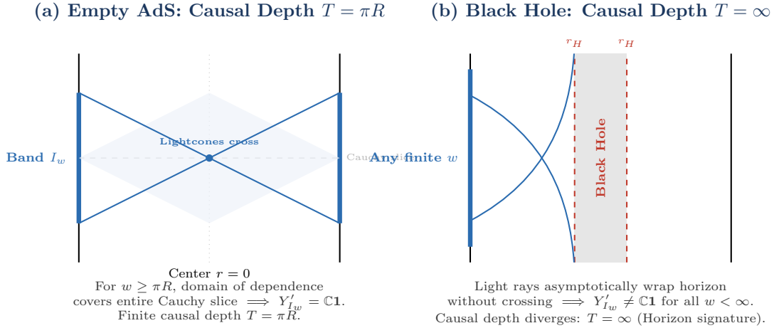
Figure 13: The causal depth parameter T(t) as an algebraic detector of horizons. (a) In empty AdS, a boundary time band I_w of width w \geq \pi R sends light rays that meet at the bulk center r = 0 and cover an entire Cauchy slice, driving the commutant to triviality ( Y'_{I_w} = \mathbb{C}1 ) and giving a finite causal depth T = \pi R . (b) In a black hole spacetime, boundary light rays asymptotically wrap around the horizon without crossing, so Y'_{I_w} \neq \mathbb{C}1 for all finite w . The causal depth diverges: T = \infty , serving as a purely algebraic boundary diagnostic of a horizon.
