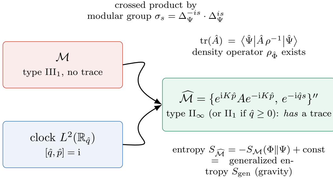
Figure 9: The crossed product construction: crossing a Type \text{III}_1 algebra \mathcal{M} (which has no trace) with its modular automorphism group \sigma_s = \Delta_\Psi^{-is} \cdot \Delta_\Psi^{is} via an auxiliary quantum observer clock L^2(\mathbb{R}) generates a Type \text{II}_\infty factor \widehat{\mathcal{M}} = \mathcal{M} \rtimes_\sigma \mathbb{R} . The resulting algebra supports a well-defined trace \tau , density matrices, and finite generalized entropy S_{\text{gen}} .
