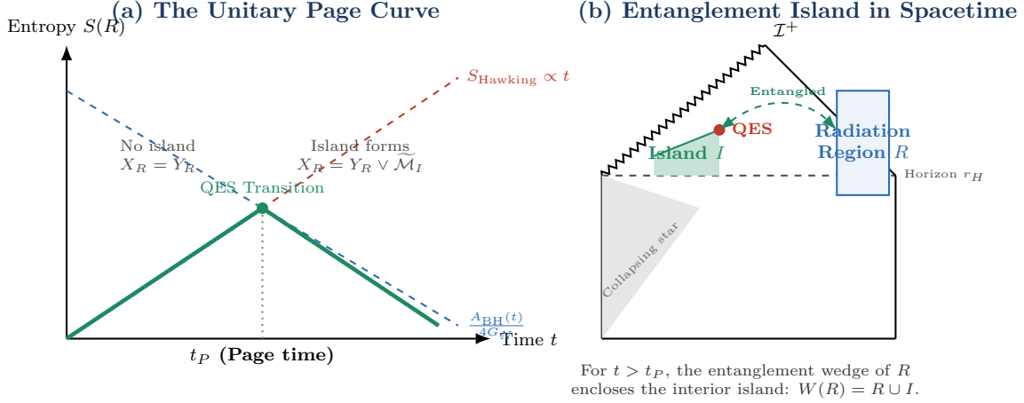
Figure 12: The Page curve and the entanglement island mechanism in an evaporating black hole. (a) Before the Page time t_P , the radiation entropy follows Hawking’s monotonically growing semiclassical curve S_{\text{Hawking}} \propto t . After t_P , a nontrivial Quantum Extremal Surface (QES) forms, and the generalized entropy is bounded by the decaying black hole area A_{\text{BH}}(t)/4G_N , restoring unitarity. (b) The Penrose diagram shows that for t > t_P , the entanglement wedge of the radiation W(R) swallows the interior island I , transferring the interior algebra \tilde{\mathcal{M}}_I into the radiation algebra: X_R = Y_R \vee \tilde{\mathcal{M}}_I .
