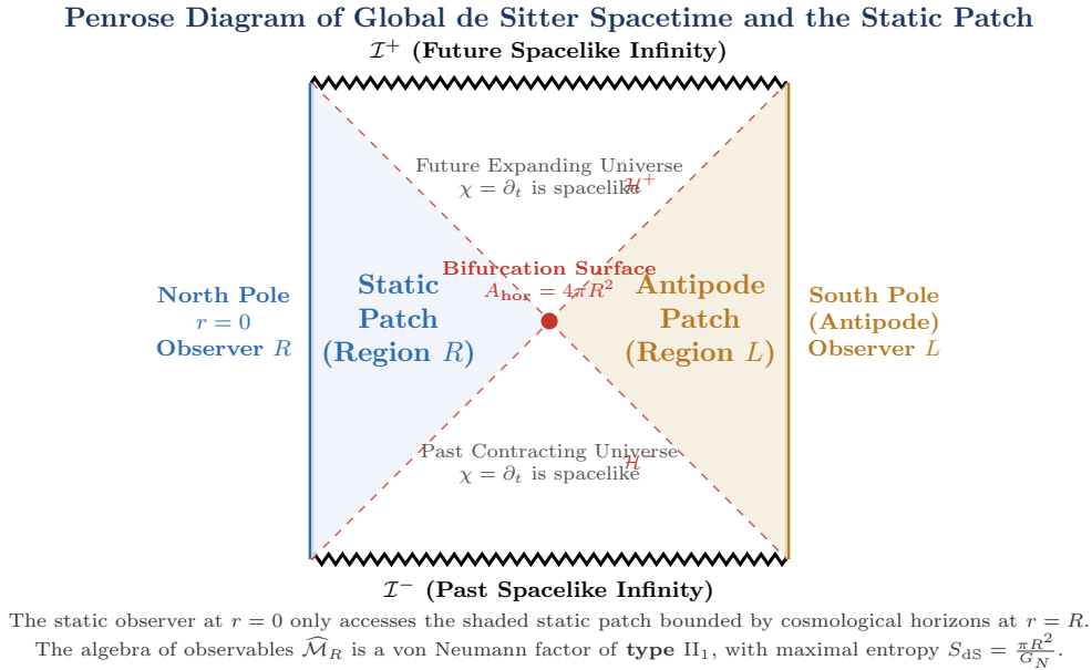
Figure 14: Penrose diagram of global de Sitter spacetime and the static patch. The static observer at the north pole r = 0 (blue trajectory) only ever accesses Region R (shaded blue), bounded by the cosmological event horizons \mathcal{H}^\pm at r = R . The south pole observer accesses the causally disconnected antipode Region L (shaded yellow). The crossed-product algebra of observables \widehat{\mathcal{M}}_R is a type \text{II}_1 factor, whose maximal entropy state is empty de Sitter.
