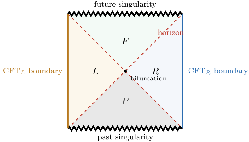
Figure 10: Penrose diagram of the two-sided eternal AdS black hole dual to the Thermofield Double state |\Psi_\beta\rangle . The right ( R ) and left ( L ) exterior wedges are causally disconnected and bounded by the event horizons (dashed red lines), connected in the interior by an Einstein–Rosen bridge (wormhole) between the past ( P ) and future ( F ) curvature singularities (zigzag lines).
