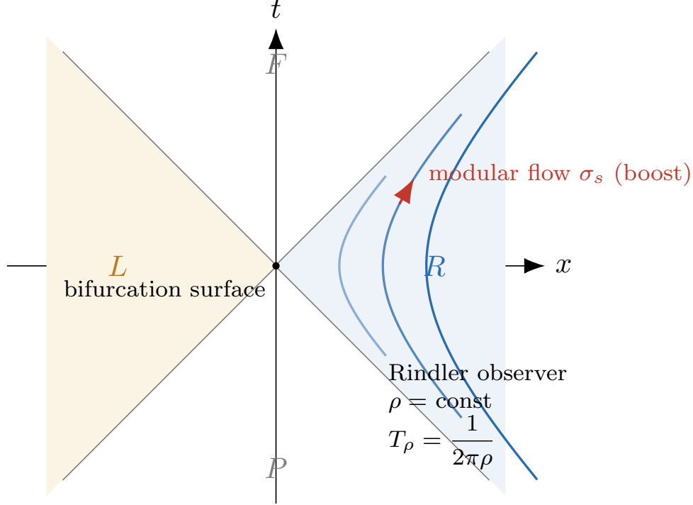
Figure 7: The spacetime geometry of the Rindler wedge: Minkowski spacetime split into the Right wedge R ( x > |t| ), Left wedge L ( x < -|t| ), Future F , and Past P . The boost hyperbolae x^2 - t^2 = \rho^2 represent trajectories of uniformly accelerated observers with proper acceleration a = 1/\rho , whose proper time \tau = \rho\eta is governed by the boost parameter \eta .
