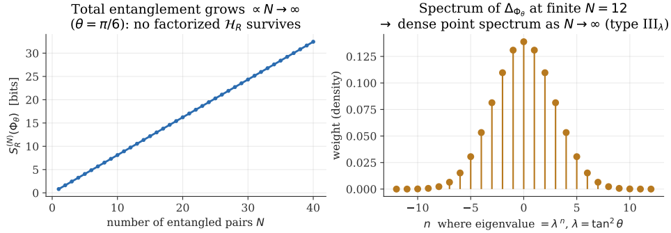
Figure 5: The emergence of non-Type I factor structures from an infinite spin chain: as the number of entangled qubit pairs N \rightarrow \infty , the discrete eigenvalues of the reduced state merge into a continuous spectrum. At \theta = \pi/4 , the algebra becomes the hyperfinite Type \text{II}_1 factor where projections span a continuous dimension range d(P) \in [0, 1] . For generic \theta \in (0, \pi/4) , the modular operator spectrum spans geometric powers \lambda^k = (\tan^2 \theta)^k , forming a Type \text{III}_\lambda factor.
