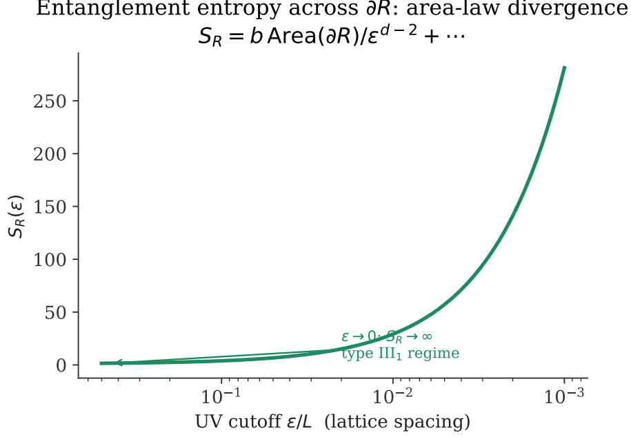
Figure 3: The UV area-law divergence of entanglement entropy in quantum field theory: dividing space across a boundary \partial R couples short-distance modes across the cut with UV cutoff \epsilon . The leading entanglement entropy diverges as S_R \sim \text{Area}(\partial R)/\epsilon^{d-2} , reflecting the infinite entanglement of the underlying Type III 1 local algebra.
