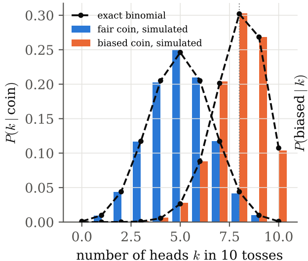
prediction: coin \rightarrow outcomes
