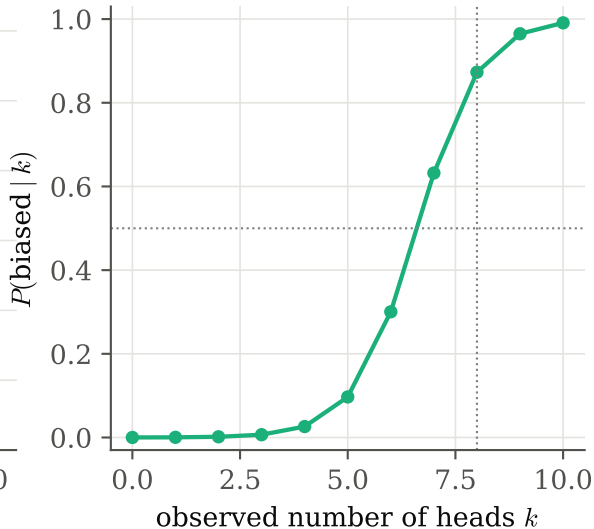
inference: outcome \rightarrow coin
