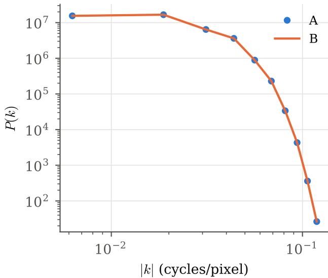
power spectra coincide
