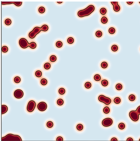
power spectra coincide
