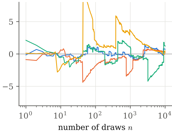
Cauchy 1/[\pi(1 + x^2)]
