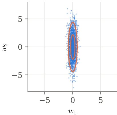
W = R^T X : diagonal
