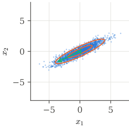
X : covariance C
