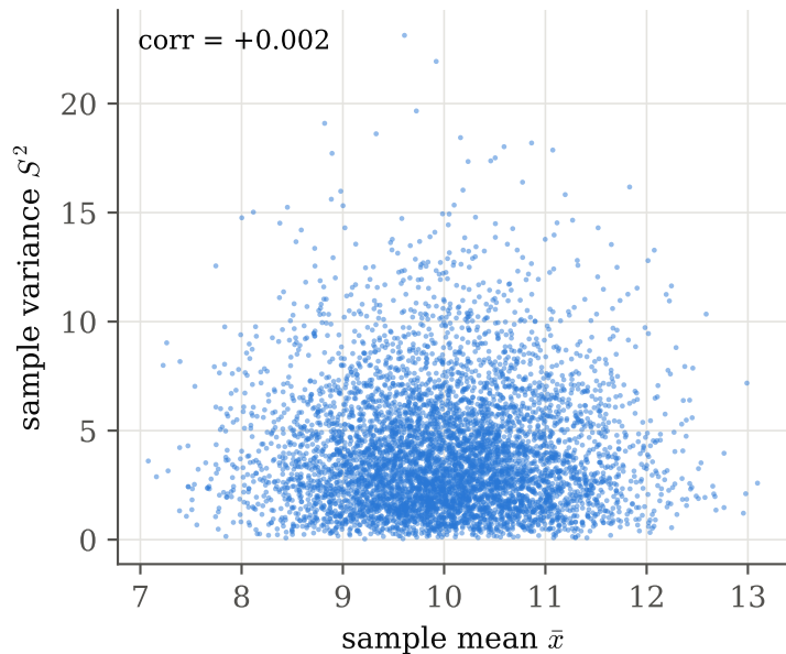
(b) \bar{x} and S^2 for a Gaussian parent
