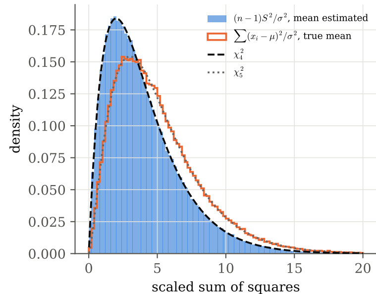
(a) n = 5 Gaussian measurements
