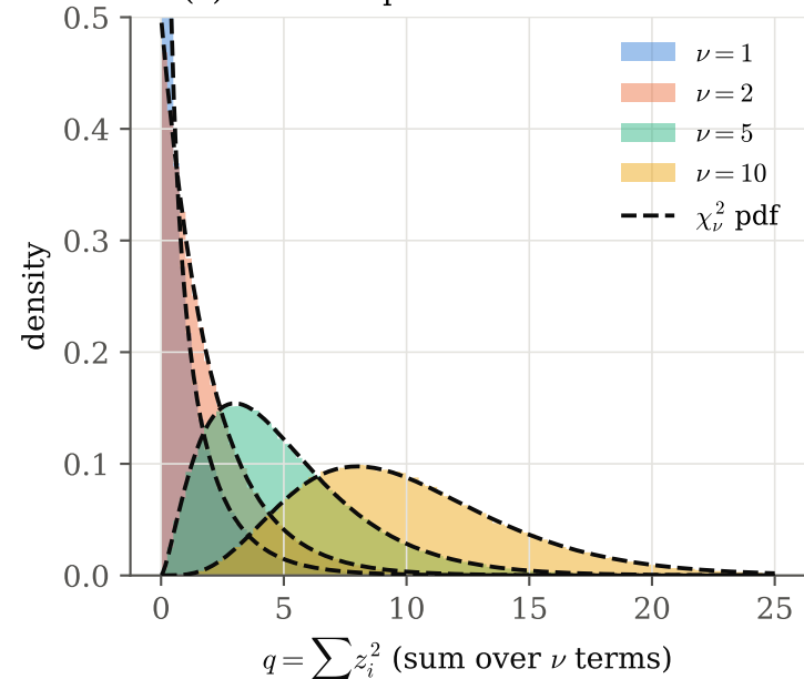
(a) sums of squared standard normals
