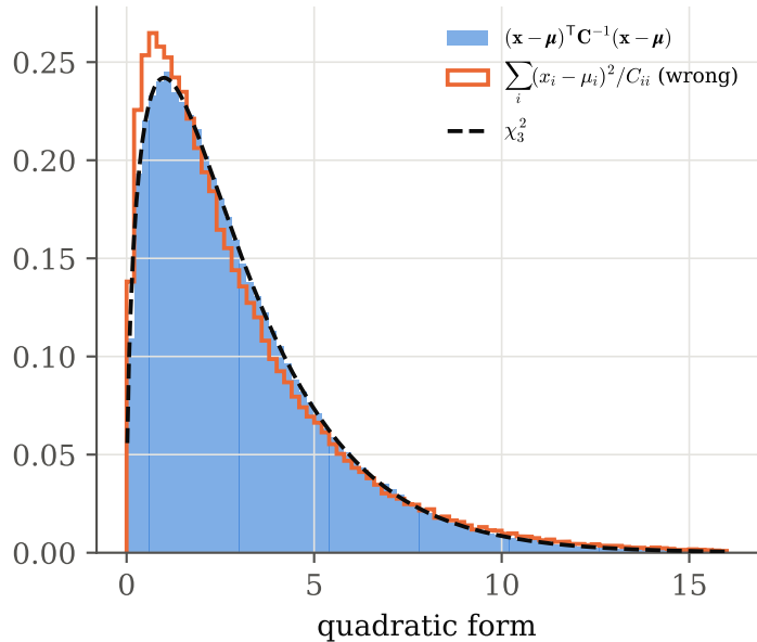
(b) correlated 3-D Gaussian
