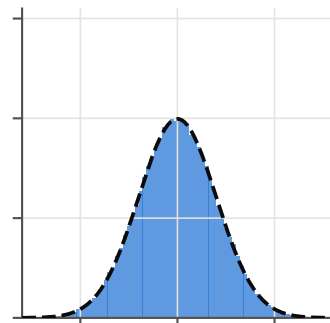
exponential, n = 30
