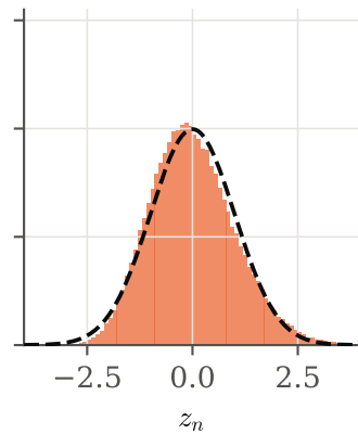
exponential, n = 30
