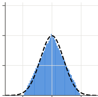
exponential, n = 2
