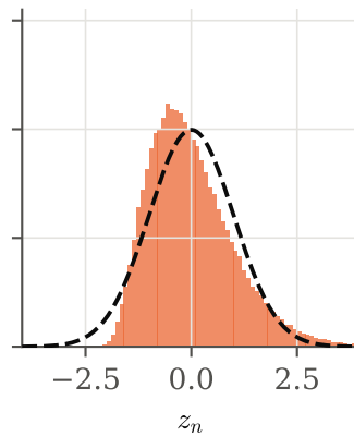
exponential, n = 5
