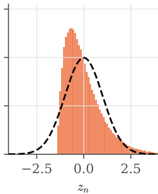
exponential, n = 2
