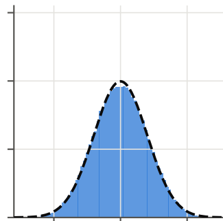
exponential, n = 5
