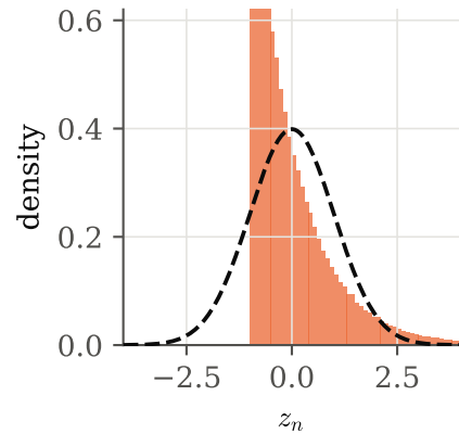
exponential, n = 1
