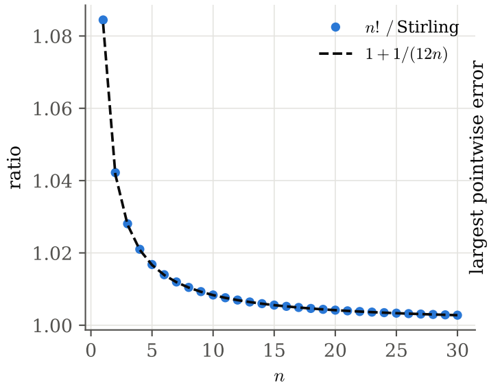
(a) Stirling's formula
