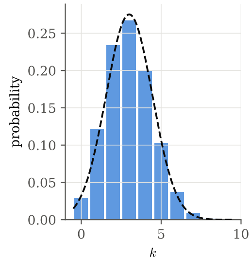
n = 10, p = 0.3
