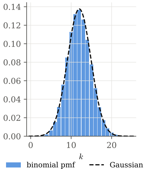
n = 40, p = 0.3
