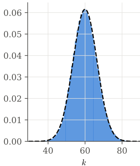
n = 200, p = 0.3
