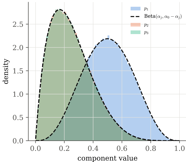
(b) each component is a Beta
