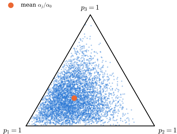
(a) Dirichlet(4, 2, 2) on the simplex
