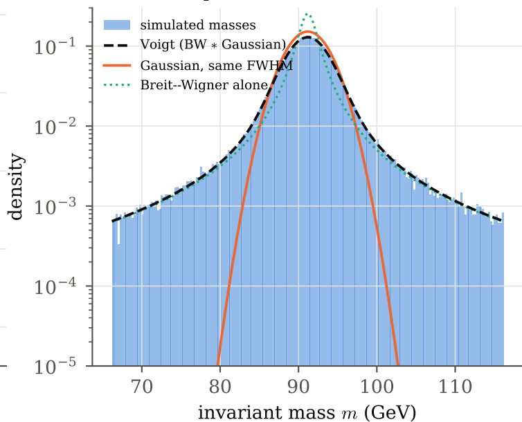
(b) a Z peak with detector resolution
