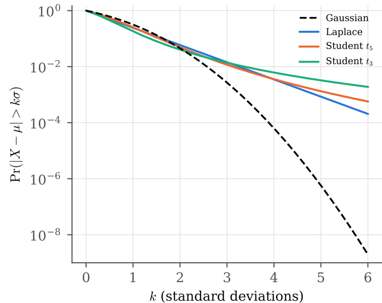
(a) same mean and variance, different tails
