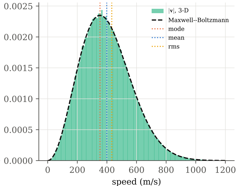
(b) argon at T = 300 K
