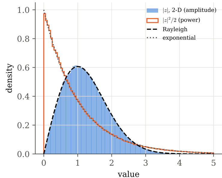
(a) a complex Gaussian mode
