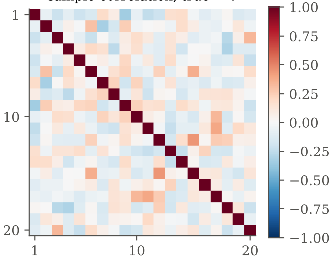
sample correlation, true = 1
