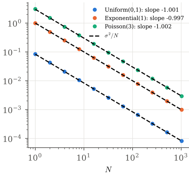
Var( \bar{X}_N ) over repetitions
