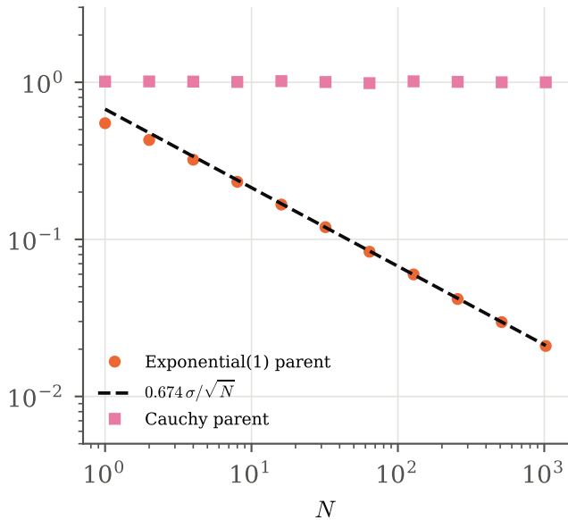
half-width of central 50% of \bar{X}_N
